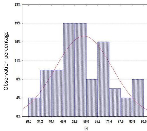
Fig. 12. Histogram of the annual number of service and repair orders for the tested systems of Autosan Sancity 12LF, 1 vehicles – density function matches empirical data Source: [Own elaboration].
