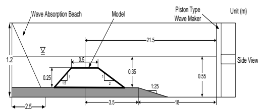
Fig. 1. Submerged breakwater model in the wave flume.
