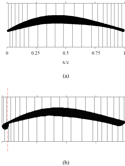
Fig. 4. The pressure taps locations on the surfaces of: (a) clean blade (Pouryoussefi et al. 2010); and (b) iced blade
