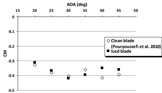
Fig. 14. The moment coefficient variation due to angle of attack changes
