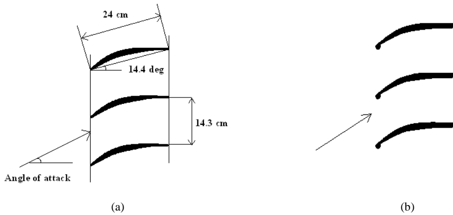
Fig. 2. Schematic view of the cascade of stator blades (experimental set-up in the wind tunnel): (a) clean blades (Pouryoussefi et al. 2010); and (b) iced blades
