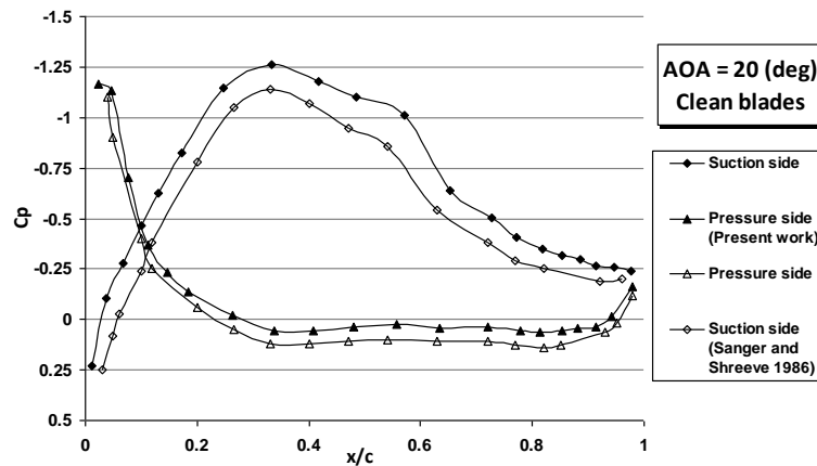
Fig. 5. Comparison of the pressure coefficient distribution with Singer and Shreeve (1986) experimental results
