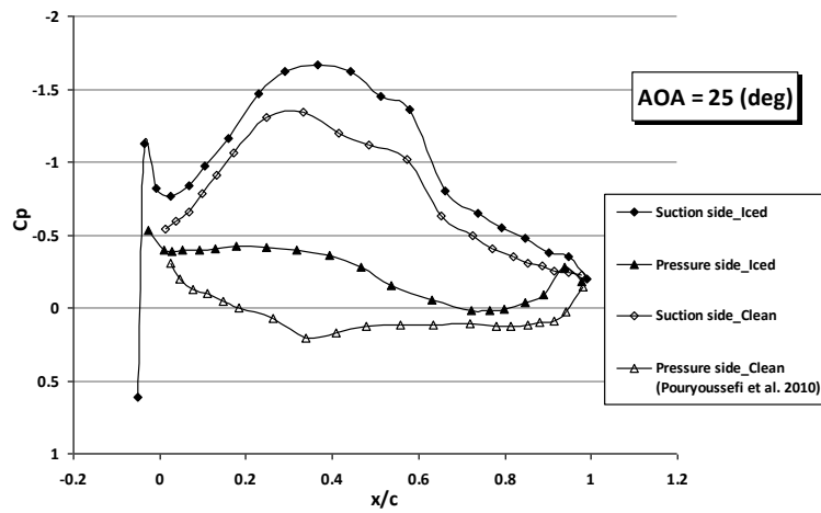
Fig. 7. The pressure coefficient distribution on the blade surface at 25°
