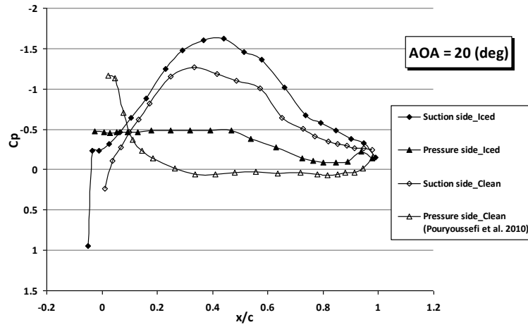
Fig. 6. The pressure coefficient distribution on the blade surface at 20°
