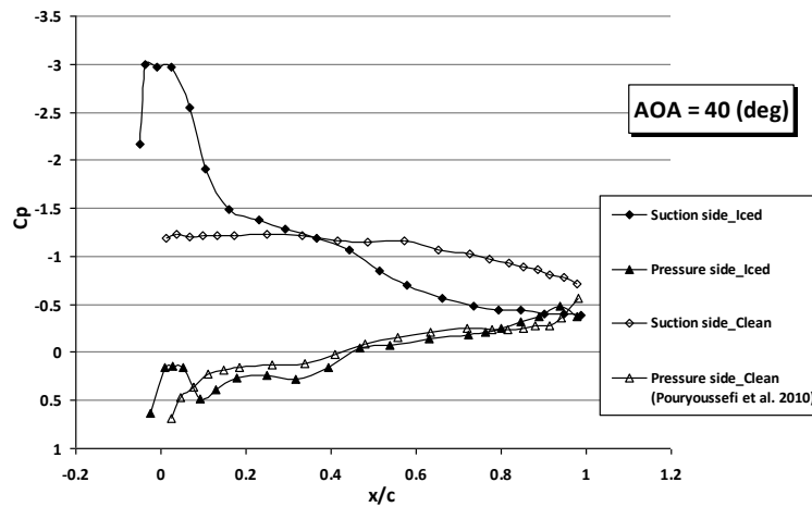
Fig. 10. The pressure coefficient distribution on the blade surface at 40°
