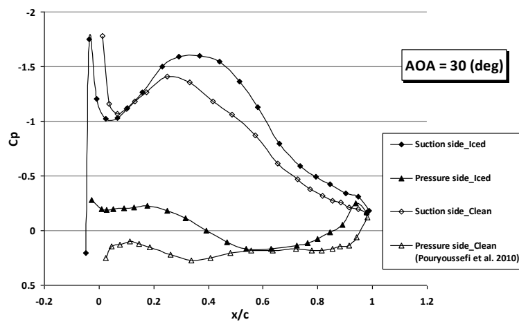
Fig. 8. The pressure coefficient distribution on the blade surface at 30°
