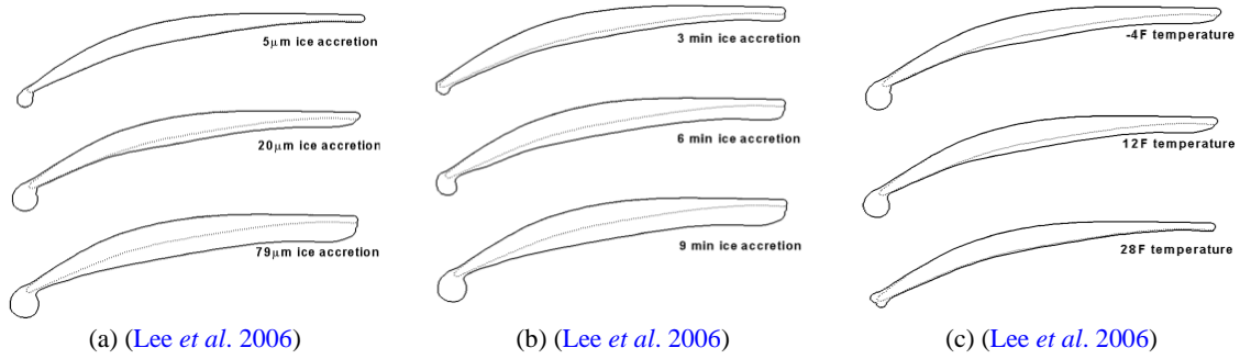
Fig. 1. Ice accretion shapes: (a) for different droplet size; (b) at 3 min intervals; and (c) for different temperatures.
