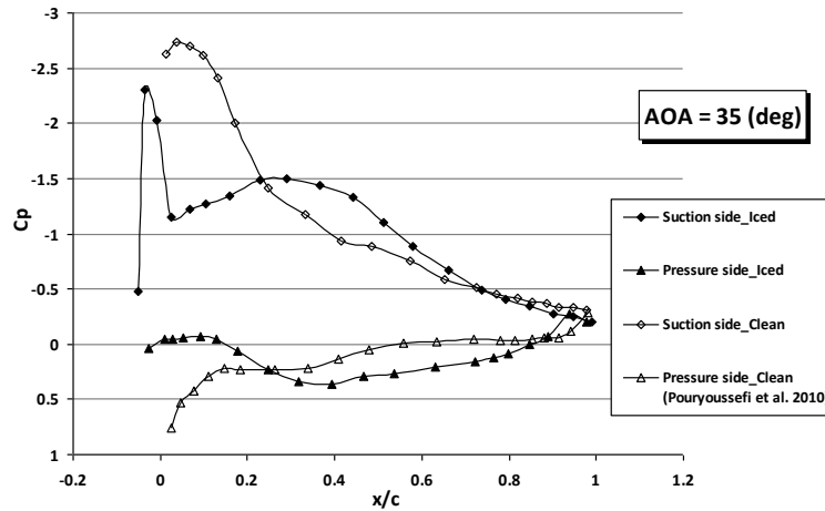
Fig. 9. The pressure coefficient distribution on the blade surface at 35°
