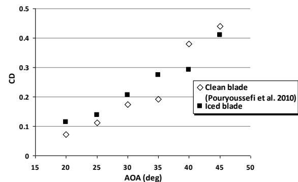
Fig. 13. The drag coefficient variation due to angle of attack changes
