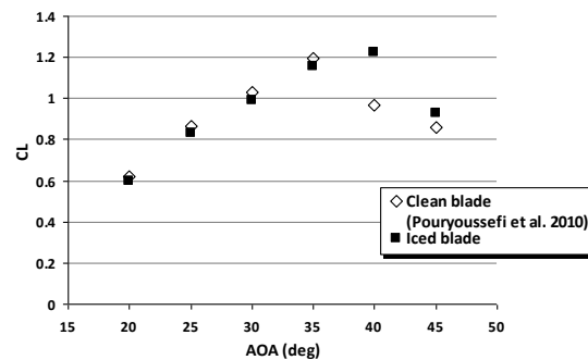
Fig. 12. The lift coefficient variation due to angle of attack changes
