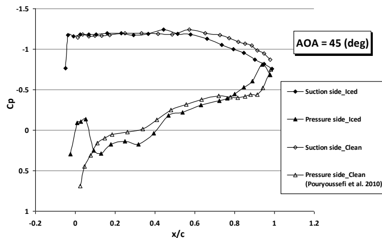
Fig. 11. The pressure coefficient distribution on the blade surface at 45°
