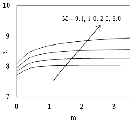
Fig. 9. The skin friction ' \tau_x ' versus 'm' for \Omega = 0.4, t = 1.0
