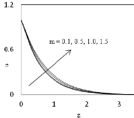
Fig. 4. The primary velocity 'u' versus 'z' for M = 1.0 , \Omega = 0.4 , t = 1
