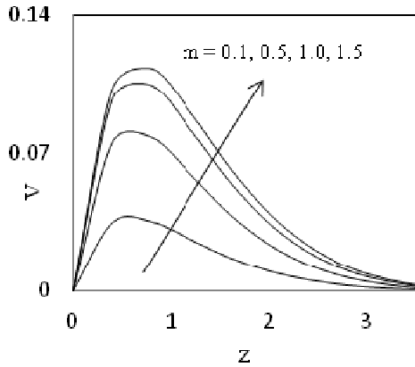
Fig. 7. The secondary velocity 'v' versus 'z' for M = 1.0, \Omega = 0.4, t = 1
