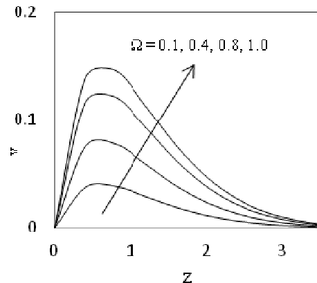
Fig. 5. The secondary velocity 'v' versus 'z' for M = 1.0 , m = 0.5 , t = 1
