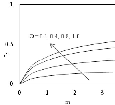
Fig. 10. The skin friction ' \tau_y ' versus 'm' for M = 1.0, t = 1.0 .
