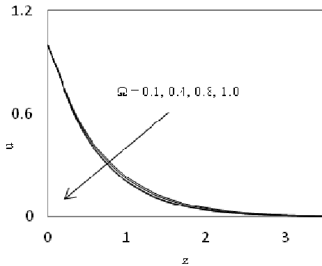
Fig. 2. The primary velocity 'u' versus 'z' for M = 1.0 , m = 0.5 , t = 1
