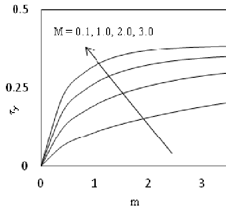
Fig. 11. The skin friction ' \tau_y ' versus 'm' for \Omega = 0.4, M = 1.0, t = 1.0
