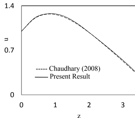
Fig. 12. Comparison of primary velocity 'u' versus 'z' for m = 0.5, M = 1.0, \Omega = 0.4 and t = 1.0 .
