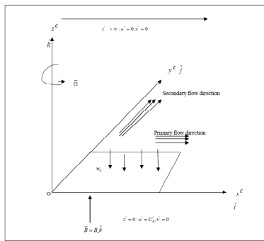
Fig. 1. Flow configuration
