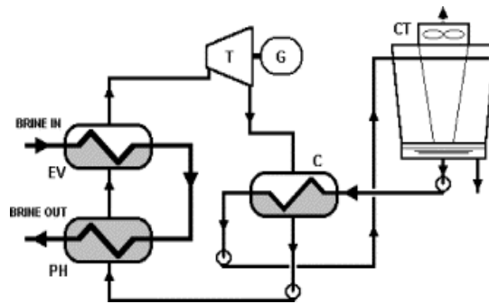
Fig. 2. Nigoricawa geothermal ORC plant (brine temperatures: inlet 140 °C, outlet 92 °C; brine flow rate 50 kg/s) ( DiPippo 2004 )
