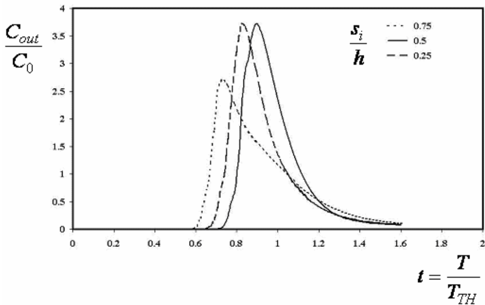
Fig. 7- FTC for different values of S_i / h .
