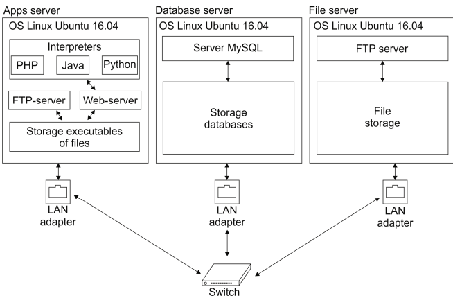
Fig. 3. General hardware and software organization of servers
