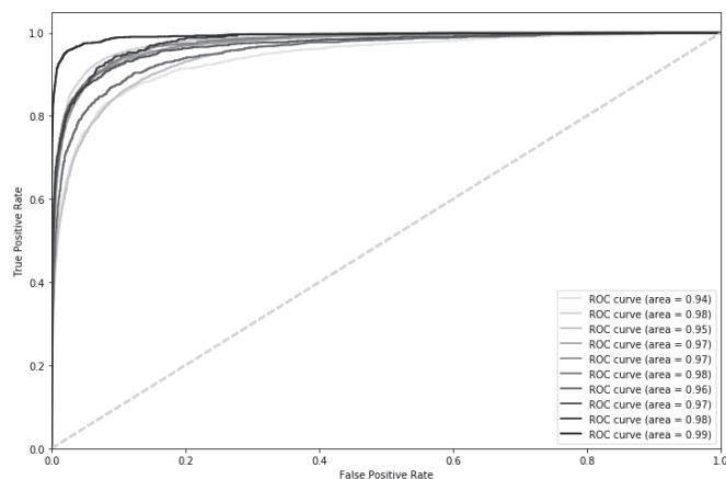
Fig. 9: ROC curves of 10 Gradient Boosting classifiers in 1-vs-Rest classification of 10 users
