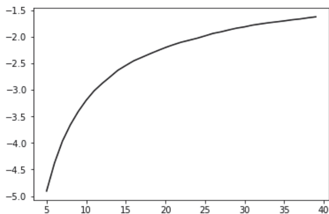
Fig. 8: Negative log loss of a KNN classifier depending on the number of the neighbours
