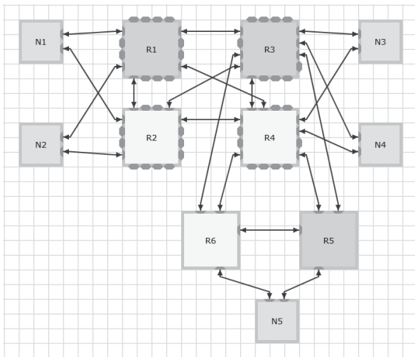
Fig. 6. Topology for tracking of routes
