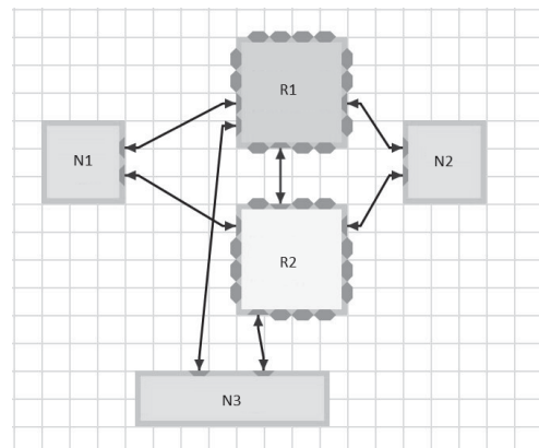
Fig. 12. SpaceWire network topology for the simulation
