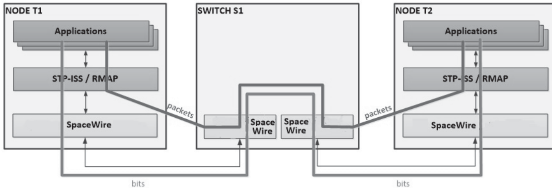
Fig. 11. Two simulation modes in SANDS
