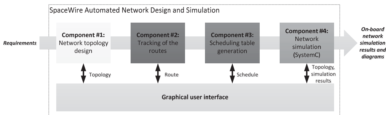
Fig. 1. Architecture of SpaceWire Automated Network Design and Simulation toolset
