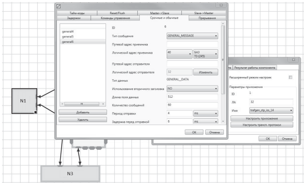
Fig. 13. Setting of traffic generator parameters
