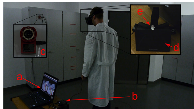
Fig. 1 System setup. a Computer system, b Oculus control box connected to the computer via USB (rotational information) and HDMI (video) connections, c wall-mounted tracker, d Oculus rift head mount, e optical marker for positional information
