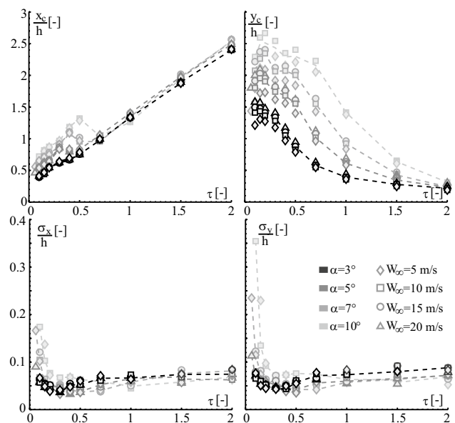
Fig. 15 Evolution of the vortex center position (top) and wandering amplitude (bottom) with the normalized clearance \tau . The dashed lines are the mean values for each incidence angle. The x -direction is represented on the left-hand side, while the y -direction is on the right-hand side
