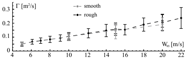
Fig. 8 Evolution of the vortex circulation with the inlet velocity for the rough and smooth hydrofoils, incidence = 5°, τ = 1.5, z/c = 1
