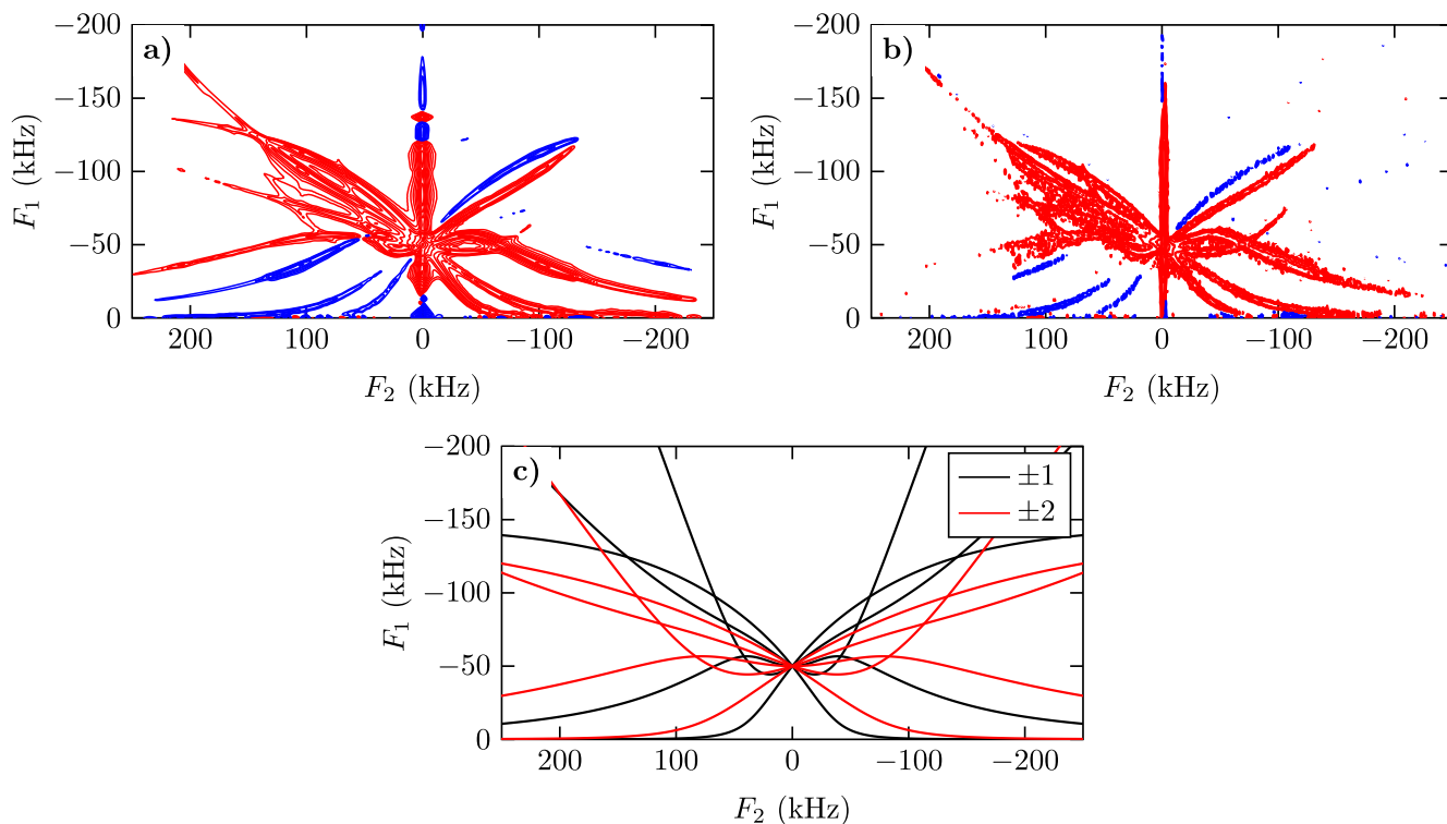
Fig. 8. Simulated (a) and experimental (b) {}^{55}\text{Mn} whole echo SATURN spectra of \text{KMnO}_4 powder recorded with 50 kHz RF at 9.4 T. (c): Simulated positions of the single quantum nutation resonances, displaying the signals due to the \pm 1 and \pm 2 satellite transitions. Note that the pattern for the \pm 2 satellites is identical to those of the \pm 1 satellites, but stretched with a factor two along the x-axis.
