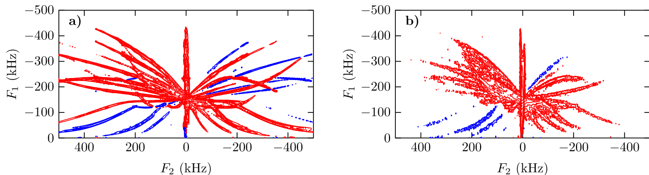
Fig. 10. Simulated (a) and experimental (b) ^{51}\text{V} SATURN spectra of \text{BiVO}_4 using 154 kHz RF power at 9.4 T.
