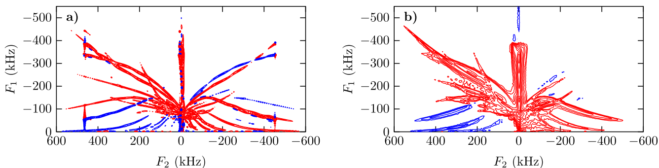
Fig. 11. Simulated (a) and experimental (b) ^{93}\text{Nb} SATURN spectra of \text{LiNbO}_3 using 78 kHz RF power at 20 T.
