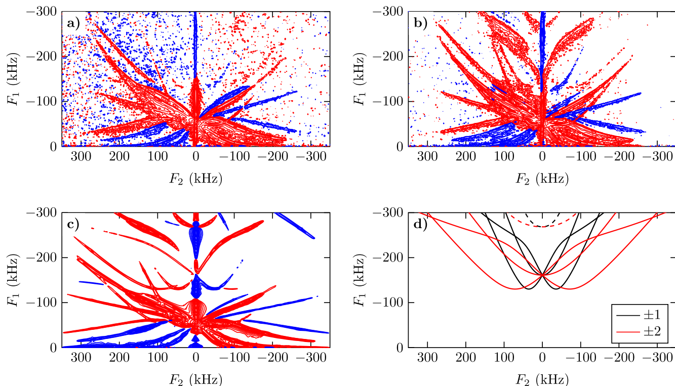
Fig. 9. ^{55}\text{Mn} whole echo SATURN spectra of \text{KMnO}_4 with 53.7 kHz RF at 14.1 T. (a): experimental without pre-inversion of the CT. (b): with pre-inversion. (c): simulation with ideal pre-inversion (negative lines coming from the top are due to aliasing). (d): 3Q (full) and 5Q (dashed) nutation transition energies for the \pm 1 and \pm 2 satellites. Also here, the pattern for the \pm 2 satellites is stretched with a factor two along the x-axis with respect to the pattern of the \pm 1 satellites.
