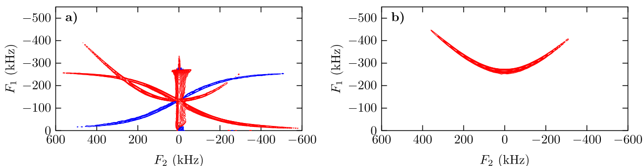
Fig. 12. Simulated SATURN spectra of a ^{23}\text{Na} Czjzek site with a small (left, 2 MHz) and high (right, 10 MHz) \sigma -value using 133 kHz RF power at 9.4 T.
