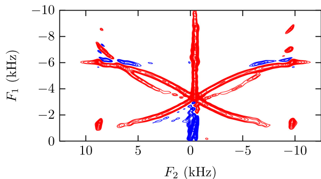
Fig. 7. {}^7\text{Li} SATURN spectrum of \text{LiBH}_4 at 110^\circ\text{C} recorded using 3.3 kHz RF field strength at 7.4 T. In this case, regular echo detection and real Fourier transform have been used (compare to Fig. 5a).
