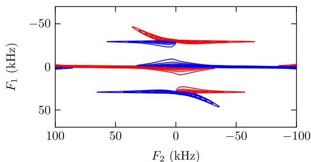
Fig. 6. SATURN spectrum of a CSA pattern ( \eta = 1 ) using 30 kHz RF. Note the offset dependent nutation frequency, the dispersive components along F_2 , and the substantial intensity around F_1 = 0 .
