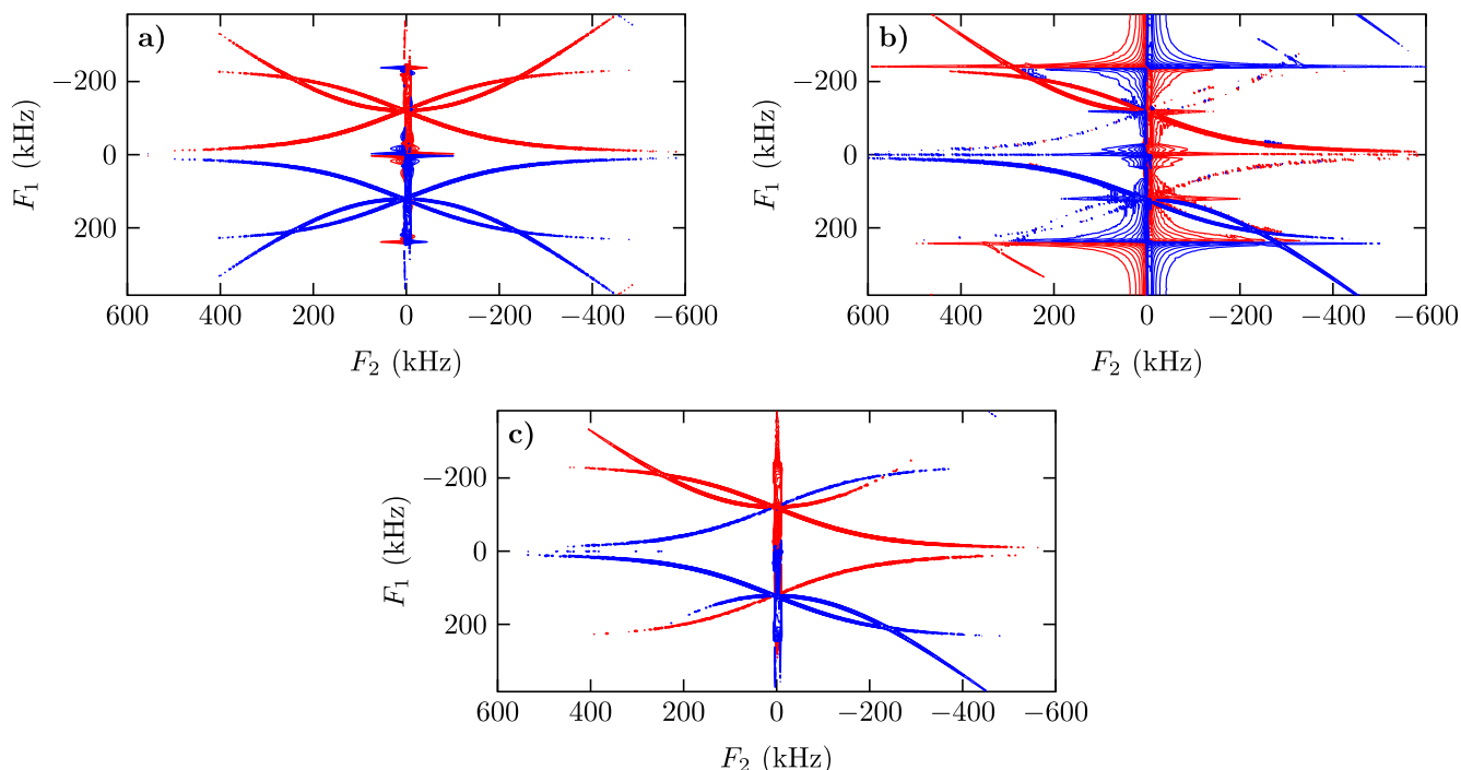
Fig. 5. Simulated ^{23}\text{Na} solid echo SATURN spectra of \text{Na}_2\text{SO}_4 ( C_Q = 2.6 MHz, \eta = 0.58 ) at an RF field strength of 133 kHz RF at 9.4 T. (a): regular echo with real Fourier transform. (b): regular echo with complex Fourier transform. (c): whole echo with complex Fourier transform.
