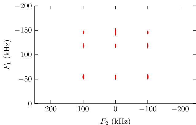
Fig. 4. 2D nutation spectrum of a I = 3/2 nucleus in a single crystal having \Omega_Q = 100 kHz using a RF field strength of 100 kHz. Only the F_1 < 0 part is shown.
