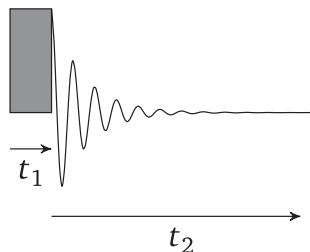
Fig. 1. Pulse sequence of a nutation experiment.
