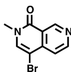
Chemical structure 1. 4-bromo-2-methyl-2,7-naphthyridin-1(2H)-one.
