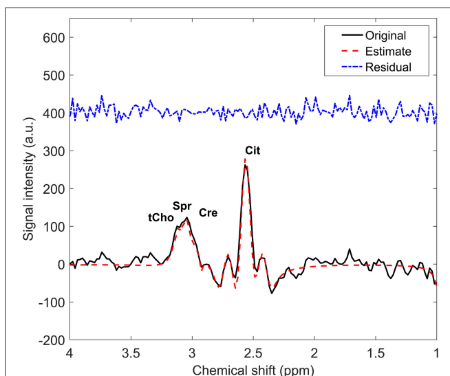
FIGURE 1 | Example of a proton MR spectrum (solid line) of one voxel in healthy prostate tissue with the overlaid spectrum fit (red dash line) and the residuals (blue dash-dot line). tCho, total choline; Spr, spermine; Cre, creatine; Cit, citrate.
