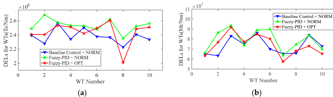
Figure 15. DELs of the WTs using Baseline Control + NORM, Fuzzy-PID + NORM and Fuzzy-PID + OPT when load B is used to test the overall controller. (a) DELs for Shaft Torsion Moment of the WTs; (b) DELs for Tower Bending Moment of the WTs.
