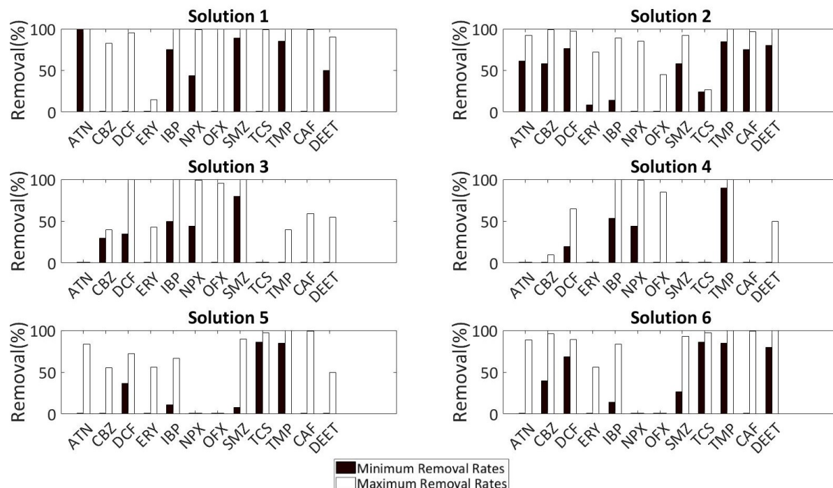
Figure 9: Percentage of CECs removed from the different treatment solutions produced from WiSDOM-CEC for Tamil Nadu.
