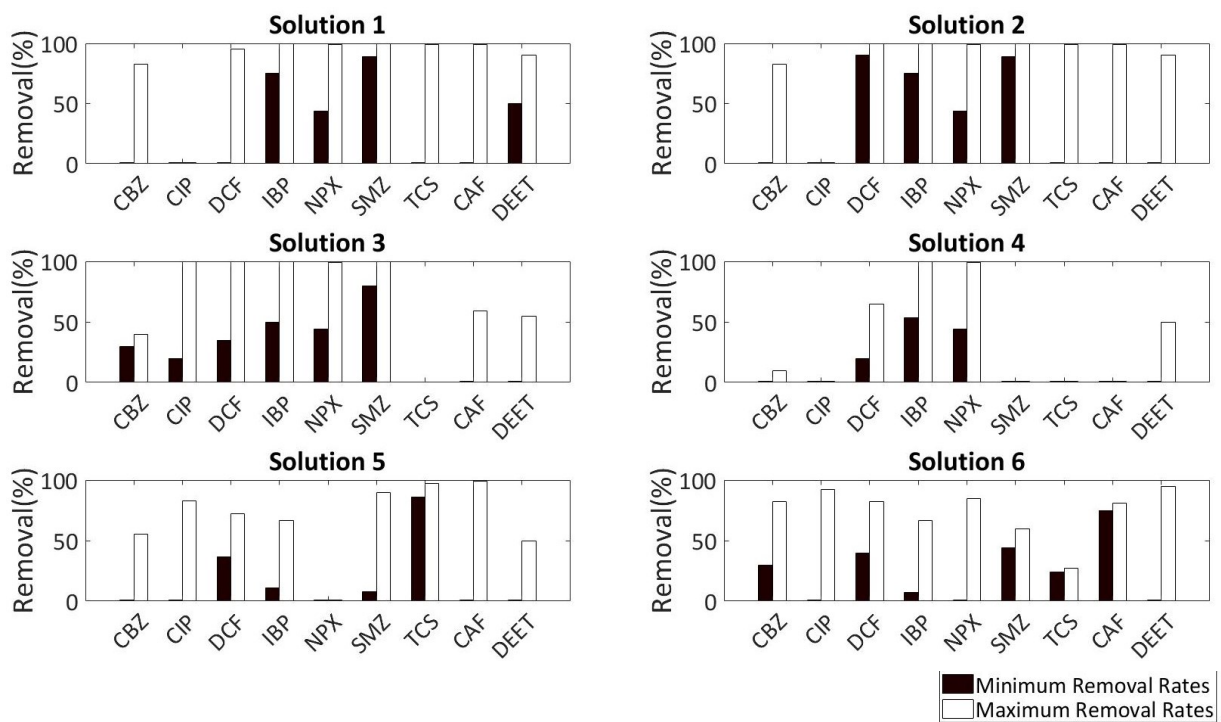
Figure 3: Percentage of CECs removed from the different treatment solutions produced from WiSDOM-CEC for Uttar Pradesh.
