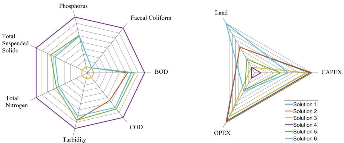
Figure 4: Performance results from WiSDOM. (Left) Radar plot from the MOO optimisation for the results for the performance of the removal of conventional pollutants for all solutions. The higher the point on the axis the worse the solution has performed. (Right) Radar plot from WiSDOM from the MOO optimisation for the results
