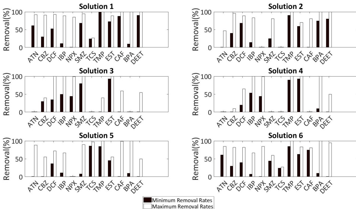
Figure 7: Percentage of CECs removed from the different treatment solutions produced from WiSDOM-CEC for Karnataka.
