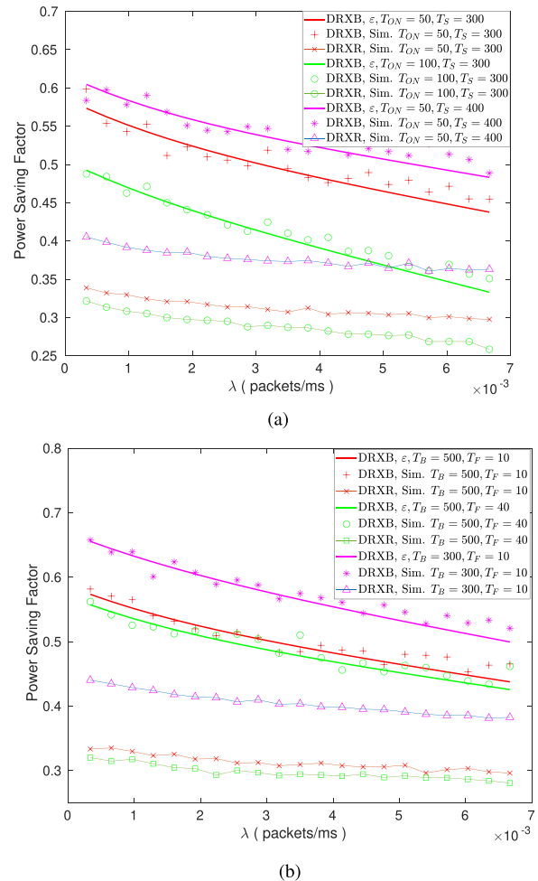
FIGURE 7. Power Saving Factor versus data arrival rate. (a) Comparison for different On Duration lengths and Sleep state lengths, with \alpha = \frac{1}{1000} , T_0 = 50 , T_F = 10 , and T_B = 500 . (b) Comparison for different Beam Training state and Feedback state lengths, with \alpha = \frac{1}{1000} , T_0 = 50 , T_{ON} = 50 , and T_S = 300 .
