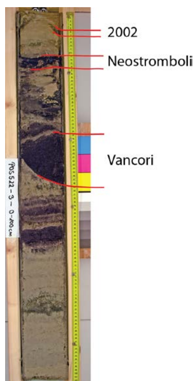
Fig. 7: Top 1 m segment of core station 3 showing major black turbidite layers with erosional unconformities.
