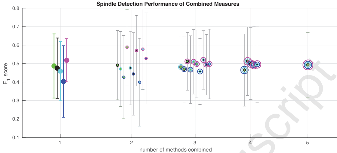
Figure 5: Combining features from the various methods. Spindle detection measures from the various tested methods were combined by taking a mean at each time point, and the agreement of these averaged measures with human scoring was evaluated via F_1 score. Two recordings with poor detector performance for all methods were omitted here. Colors correspond to the different methods, when methods are combined, concentric circles corresponding to the combined measures are plotted at one point. For all methods and combinations of methods, the mean across all recordings is shown. Error bars represent the standard deviation across recordings. Mean F_1 scores for these combinations of detectors are also shown in Table 4. It is noteworthy that there is a significant boost in detection performance only when combining DDA with any one of the spectral methods. No other combination of methods provides such a boost.
