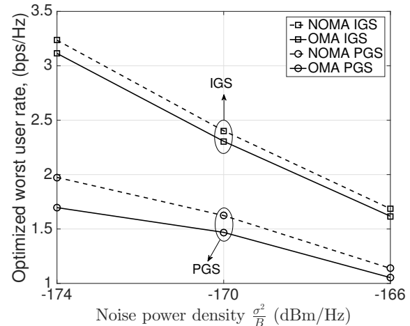
Fig. 4. Optimized worst user rate for varying values of noise power density \frac{\sigma_n^2}{B} , and fixed N_t = 6 BS antennas, K = 1 cell, N = 8 UEs, P^{\max} = 26 dBm.
