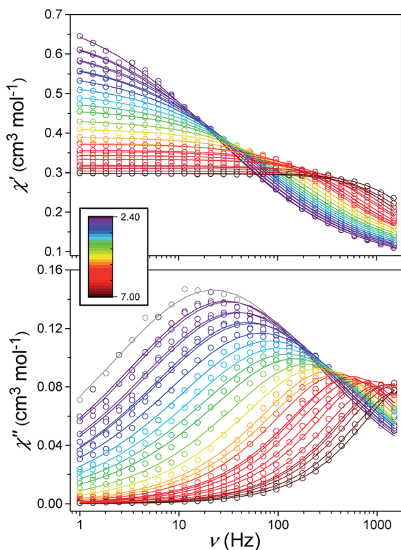
Fig. 6 Frequency-dependence of the in-phase ( \chi' ) and out-of-phase ( \chi'' ) susceptibility signal over a range of temperatures and conducted under H_{\text{dc}} = 2500 \text{ Oe} .
