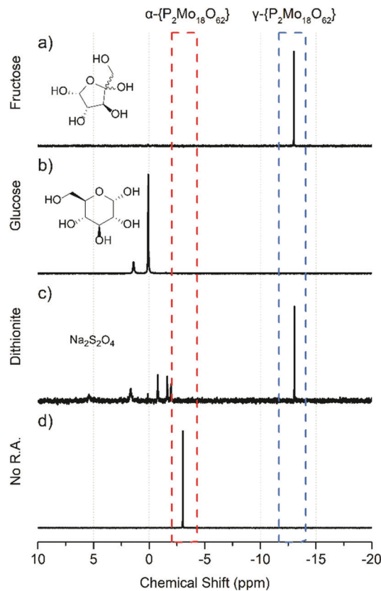
Fig. 2 ^{31}P -NMR in D_2O of isolated products of reactions containing sodium molybdate ( 100 \text{ mg mL}^{-1} ), 1 eq. H_3PO_4 , and 1.2 eq. of (a) D-(−)-fructose, (b) D-(+)-glucose, (c) sodium dithionite, or (d) no reducing agent at pH 1. All reactions stirred for 24 h at room temperature (20 °C).
