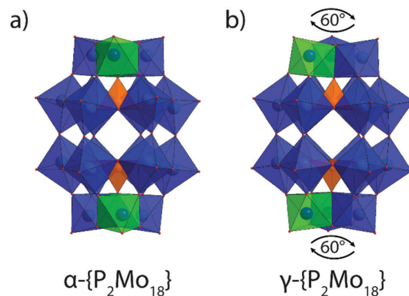
Fig. 1 Single crystal XRD structures of molybdenum Wells–Dawson structural isomers (a) \alpha - \{P_2Mo_{18}\} and (b) \gamma - \{P_2Mo_{18}\} isolated in this work. Blue polyhedra and spheres: Mo, orange polyhedra and spheres: P; red spheres: O. Note one pair of Mo polyhedra are highlighted green to visualize cap rotation difference between isomers.
