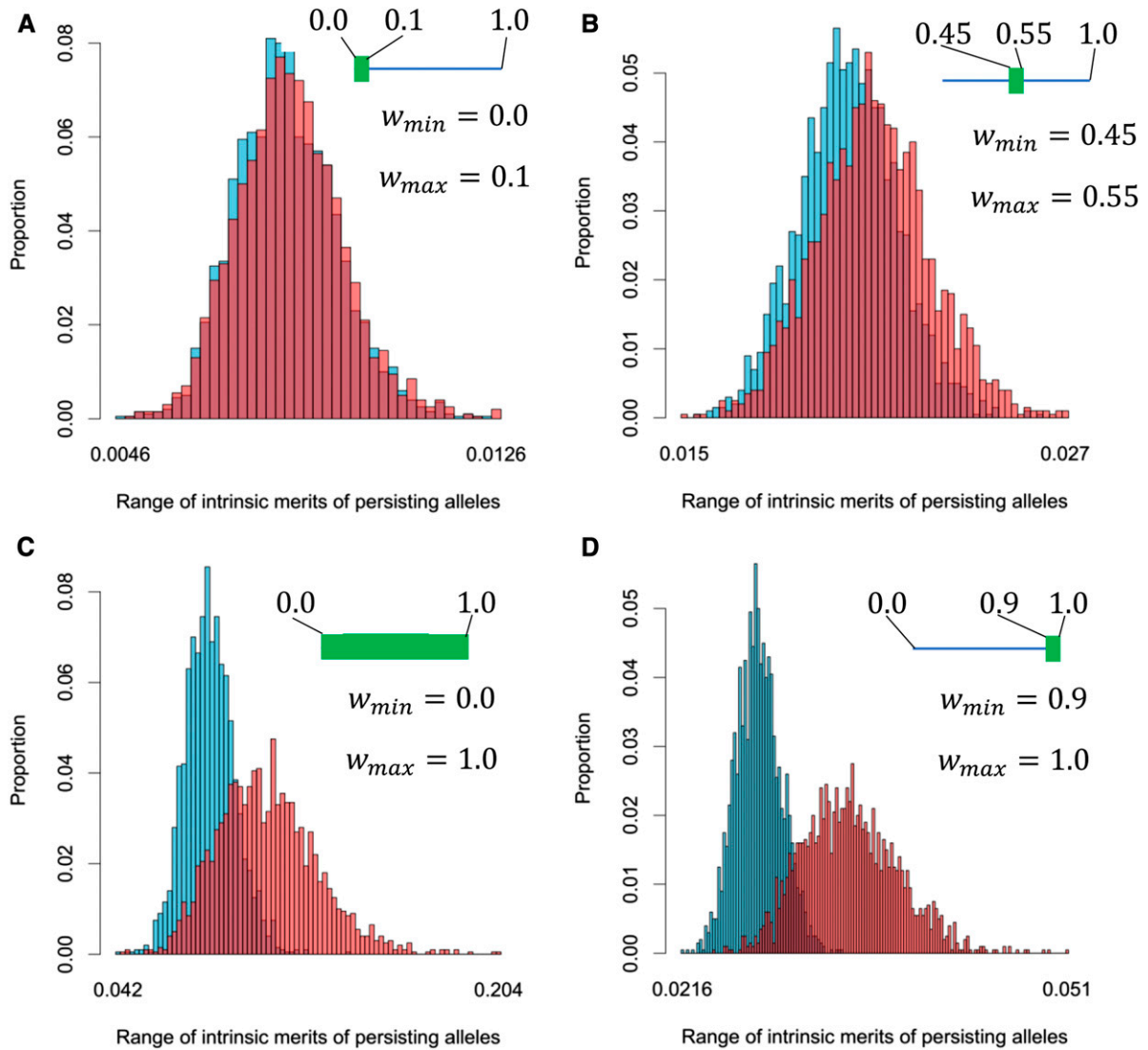
Figure 3 The range of intrinsic merits of the set of alleles maintained at equilibrium for the Random experiment and (A) scenario 3, i.e., (w_{min}, w_{max}, f, n_{ini}) = (0.0, 0.1, 2, 250) ; (B) scenario 13, i.e., (w_{min}, w_{max}, f, n_{ini}) = (0.45, 0.55, 2, 250) ; (C) scenario 63, i.e., (w_{min}, w_{max}, f, n_{ini}) = (0.0, 1.0, 2, 250) ; and (D) scenario 73, i.e., (w_{min}, w_{max}, f, n_{ini}) = (0.9, 1.0, 2, 250) . The red bars correspond to the Divergent Allele Advantage (DAA) model, while the blue bars correspond to the asymmetric overdominance (AO) model. The distribution of the ranges of intrinsic merits for the DAA model changes toward larger ranges relative to the AO model from (A), a scenario where both the initial intrinsic merit range and the maximum intrinsic merit are low, to (D), a scenario where the initial intrinsic merit range is low but the maximum intrinsic merit is high.
