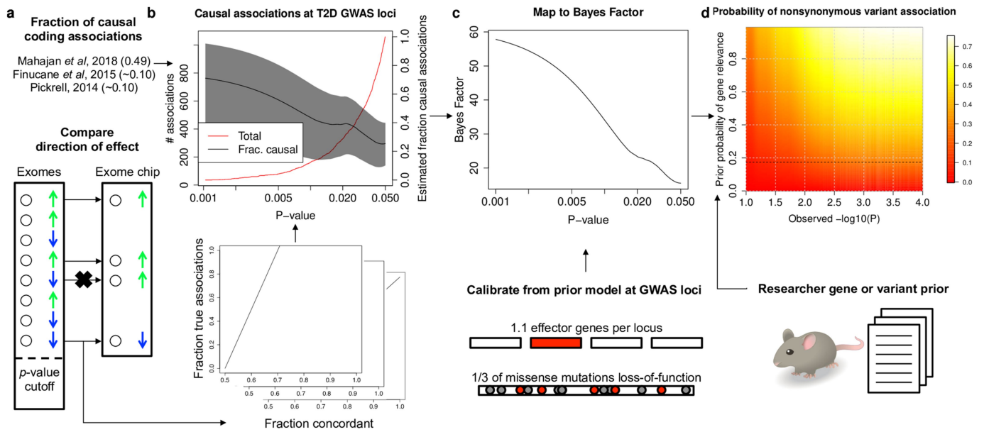
Extended Data Fig. 7 | PPA calculation workflow. a , We estimated the PPAs for nonsynonymous variants in our sequence analysis based on concordance with independent exome array data and previously published 16,78,80 estimates of the fraction of causal coding associations (Methods). b , PPA estimates for nonsynonymous variants within T2D GWAS loci are shown as a function of P value (right y axis, black line; 95% confidence interval, grey shading) together with the total number of such variants (left y axis, red line). c , For variants outside of T2D GWAS loci, we developed a method to further compute Bayes factors, which measure the odds of true and causal association, as a function of P value,
