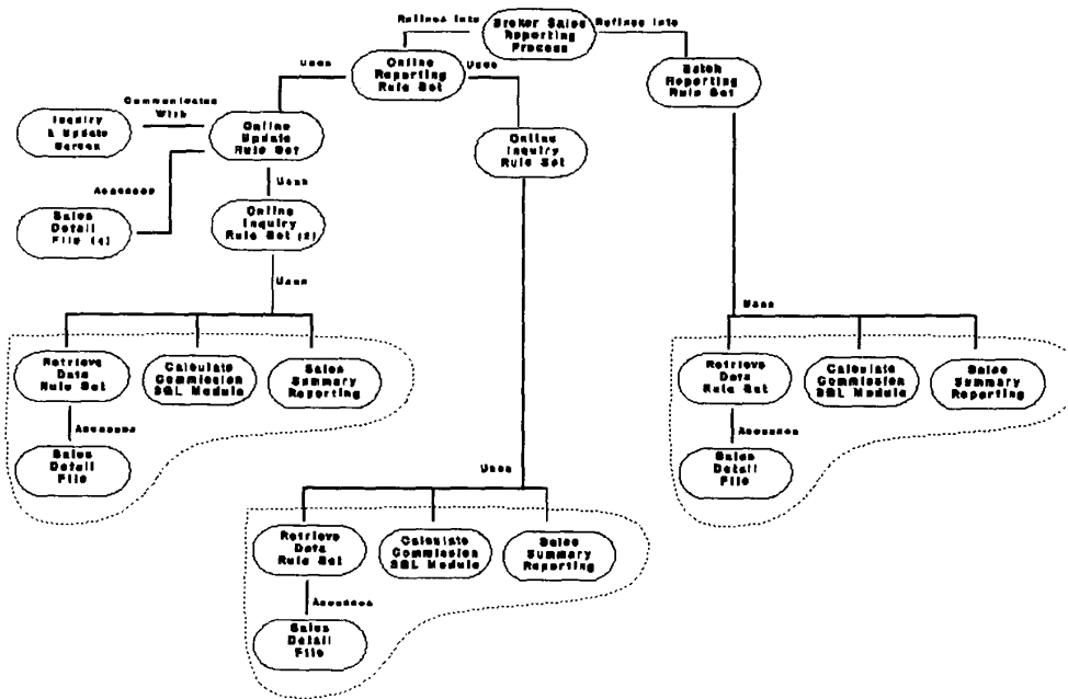
Fig. 8. Expanded hierarchy for a subset of the Broker Sales Reporting System. This figure displays the same subset as it would appear in the absence of object reuse. Several of the objects would have to be rewritten many times. Reuse Leverage is the ratio of the number of objects used (Fig. 8) to the number of unique objects actually written for this application (Fig. 7). The 3GL MODULE (Calculate Broker Commission) is external to this application; it was originally written for a different application, and reused by the programmers of this one. Therefore, the Software Reuse Analyzer will not include it in the count of unique objects written for this application.
