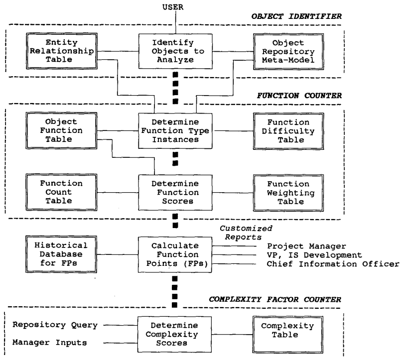
Fig. 4. The automated Function Point Analyzer: A schematic. The Function Point Analyzer consists of three subsystems. One uses the metamodel to identify the objects in the application under analysis. The second uses it to assign Function Count scores to those objects. The third obtains task complexity measures (Table III). This requires that the programmer or manager input in parallel with the automated analysis (Fig. 5).
