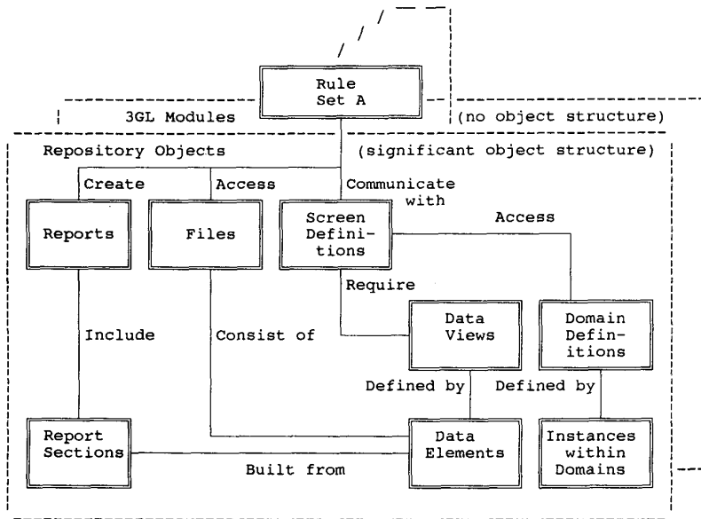
Fig. 2. ICE repository objects. This figure is an expansion of RULE SET A from Fig. 1. There is a well-defined set of relationships allowed. Each object resides in the repository, and has a descriptive entry in a database table that also resides there. In addition, the repository contains other tables with entries for each relationship between two objects. A RULE SET may also use preexisting 3GL MODULES. The repository contains no information about the processing performed by these modules. Any functionality that they provide the user, via REPORTS, FILES, or SCREENS, however, must be mediated by an ICE object.
