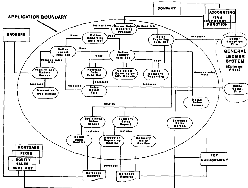
Fig. 6. The Broker Sales Reporting System: System layout. The Broker Sales Reporting System consists of those repository objects that are invoked by the Broker Sales Reporting Process, and of the relationships between those objects. The PROCESS refines into two RULE SETS, one for online processing, and one for batch processing. Since the two RULE SETS generate similar outputs, they have a number of other repository objects in common. Each such object is stored only once in the repository, and reused as necessary. Each use will be instantiated in the metamodel as an entry in the table of relationships.
