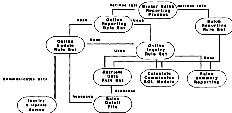
Fig. 7. A subset of the Broker Sales Reporting System.
