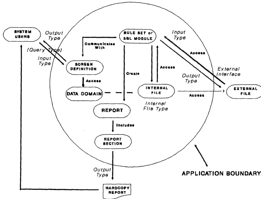
Fig. 3. Mapping from ICE objects to function counts. Function point analysis measures the functionality that a system delivers to the user in terms of data transfers into or out of that system (External Inputs, External Outputs, Queries, External Interfaces), and in terms of the data stores (Logical Internal Files) used. A 3GL program can contain functionality of all five classes. An ICE object, however, is severely constrained in the functionality that it can represent, to the point where a system's function count can be computed by identifying and classifying its objects. See Table I.
