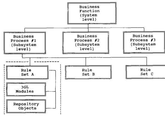
Fig. 1. A repository-based application metamodel. A BUSINESS FUNCTION is represented in ICE by a menu of BUSINESS PROCESSES. An application consists of all of the objects called (directly or indirectly) by a given BUSINESS PROCESS. The first step in analyzing a system is to identify these objects, by iteratively tracing the calling relationships stored in the metamodel. A BUSINESS PROCESS will call one or more RULE SETS. Each RULE SET, in turn, may call other RULE SETS, 3GL MODULES, or other ICE objects (Fig. 2). Note that the use of an object by an application system does not preclude its reuse by another application.
