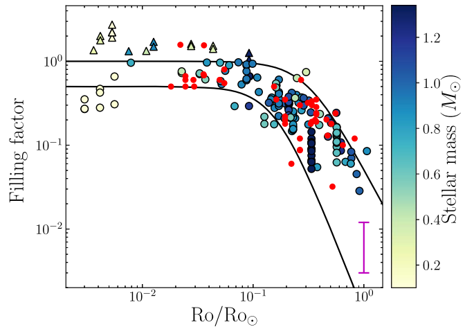
Figure 4. Filling factor against Rossby number normalized to the solar Rossby number. The data points of Cranmer & Saar (2011) are shown in red while their bounding curves are shown in black (see their figure 7(b)). The range of filling factors exhibited by the Sun, as estimated by Cranmer (2017), is shown with a magenta strut. The estimated filling factors of the ZDI sample are shown with the colored points color coded by stellar mass. Stars with estimated filling factors larger than 1 are shown with triangular points.
