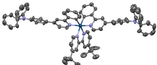
Fig. 1. Solid-state structure of complex 3a . Thermal ellipsoids are drawn at the 50% probability level. Hydrogen atoms, PF 6 - counterion and solvent molecules are omitted for clarity.
