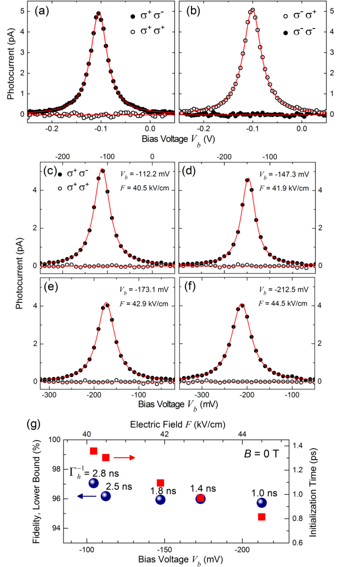
FIG. 3. (Color online) Measurement of the fidelity of hole-spin initialization. (a) X^+ PC spectra for cross- (co-) polarized laser excitation using a \sigma^+ -polarized X^0 laser, for the initialization of a spin-up hole, and a \sigma^- ( \sigma^+ )-polarized X^+ laser. High contrast is observed as the copolarized PC peak vanishes below the noise level, thereby setting a lower bound for the fidelity. (b) Analogous measurement result to (a), but for the initialization of a spin-down hole. (c)–(f) Cross- and copolarized X^+ PC spectra for a number of increasing reverse-bias voltages and for the initialization of a spin-up hole, showing similar results to (a) and (b). (g) Plot of the measured lower bounds of fidelity, along with their corresponding initialization time ( \Gamma_e^{-1} ) and hole tunneling time \Gamma_h^{-1} , as a function of V_b and F . At V_b = -212.5 mV, the initialization time is reduced below 1 ps, while the lower bound of fidelity remains high, as seen also from the high contrast in (f), and \Gamma_h^{-1} is still more than three orders of magnitude longer than \Gamma_e^{-1} to allow for a potential spin-storage efficiency of near unity.
