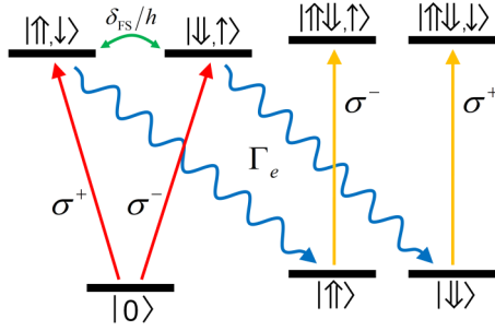
FIG. 1. (Color online) Scheme for hole-spin initialization and measurement of fidelity. Resonant excitation from the ground state |0\rangle (empty QD) to the X^0 state |\uparrow, \downarrow\rangle ( |\downarrow, \uparrow\rangle ), which consists of a spin-up (-down) hole and a spin-down (-up) electron, is achieved using a \sigma^+ ( \sigma^- )-polarized laser (straight arrows on left-hand side). Fast ionization of |\uparrow, \downarrow\rangle ( |\downarrow, \uparrow\rangle ) via electron tunneling results in the initialization of |\uparrow\rangle ( |\downarrow\rangle ) at a rate \Gamma_e (wavy arrows). Prior to electron tunneling, however, coupling between X^0 states due to fine-structure splitting at a frequency \delta_{FS}/h leads to X^0 spin dephasing and a subsequent loss in initialization fidelity. Using a second laser tuned to the X^+ transition, the fidelity of |\uparrow\rangle ( |\downarrow\rangle ) initialization is measured by comparing the probability of creating X^+ for \sigma^- ( \sigma^+ ) cross-polarized and \sigma^+ ( \sigma^- ) copolarized excitation with respect to the polarization of the first laser.
