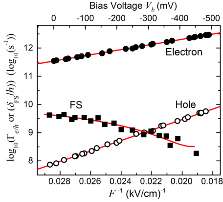
FIG. 2. (Color online) Comparison of electron tunneling rate to hole tunneling rate and fine-structure splitting. \Gamma_e is about three orders of magnitude faster than \Gamma_h throughout the measured range. Also, \Gamma_e is between two and four orders of magnitude faster than \delta_{FS}/h throughout the measured range. For \delta_{FS} , the solid curve is the difference between the quadratic fit curves of the V_b vs. energy data for the two linearly polarized X^0 eigenstates (see Supplemental Material [27]).
