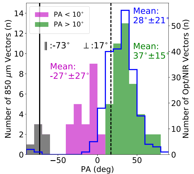
Figure 4. Histogram of the magnetic field orientations. The colored histogram shows the 850 \mu\text{m} polarimetry data, and the blue histogram represents the optical/infrared data. The bin size of the histograms is set to 10^\circ , similar to our typical uncertainties in PA. The PA = 0^\circ corresponds to north, and PA = +90^\circ is east. Our data show two major components with mean PA of -27^\circ (red) and 37^\circ (green), separated by a dip at \approx 10^\circ , and a minor component peaked at -75^\circ (gray). The black solid and dashed vertical lines label the orientation parallel and perpendicular to the large-scale filament, respectively, and the perpendicular orientation is consistent with the dip between the observed two components.
