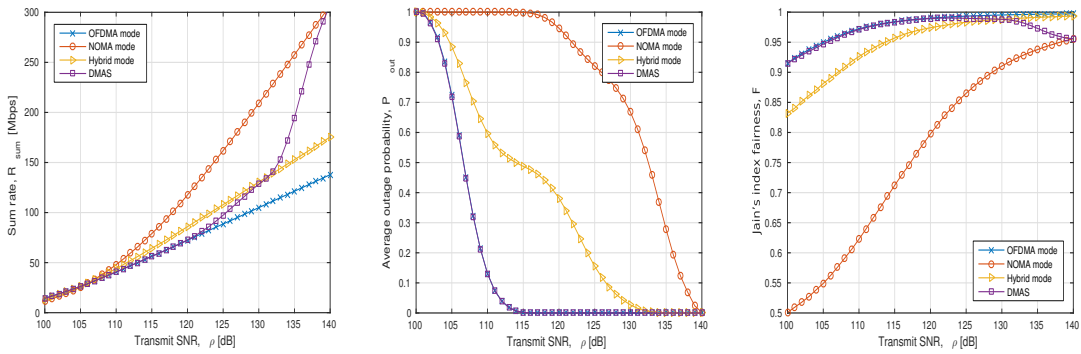
Figure 6: Achieved performance under the different MA schemes compared to the proposed DMAS with [\varpi_{R_{sum}}, \varpi_{P_{out}}, \varpi_{\mathcal{F}}] = [0.4, 0.3, 0.3] for a system with 3 multiplexed users.
