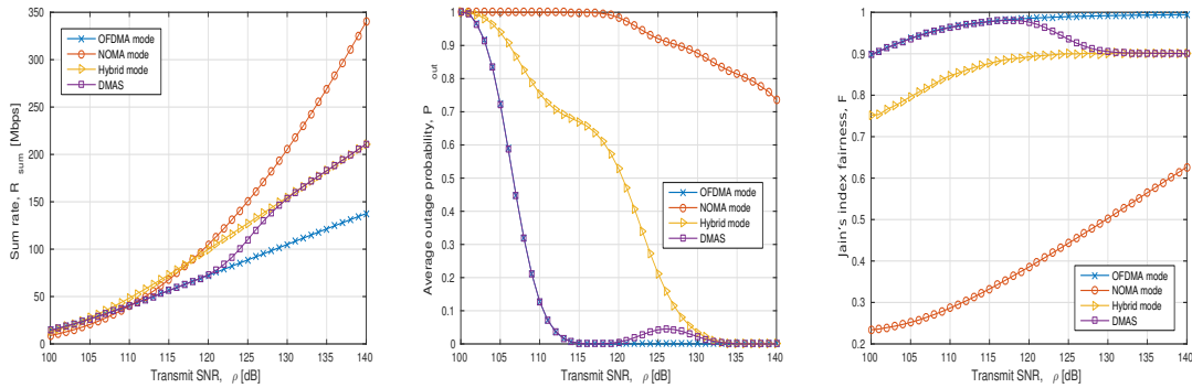
Figure 7: Achieved performance under the different MA schemes compared to the proposed DMAS with [\varpi_{R_{sum}}, \varpi_{P_{out}}, \varpi_{\mathcal{F}}] = [0.4, 0.3, 0.3] for a system with 6 multiplexed users.
