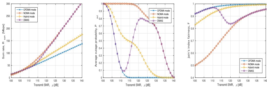
Figure 8: Achieved performance under the different MA schemes compared to the proposed DMAS with [\varpi_{R_{sum}}, \varpi_{P_{out}}, \varpi_{\mathcal{F}}] = [0.8, 0.2, 0] for a system with 3 multiplexed users.
