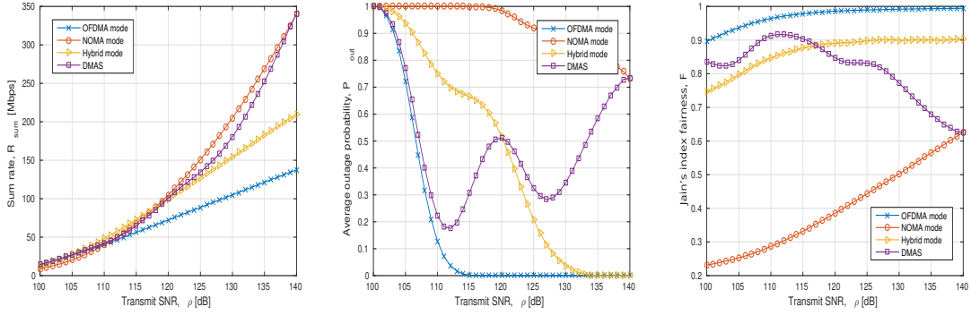
Figure 9: Achieved performance under the different MA schemes compared to the proposed DMAS with [\varpi_{R_{sum}}, \varpi_{P_{out}}, \varpi_{\mathcal{F}}] = [0.8, 0.2, 0] for a system with 6 multiplexed users.
