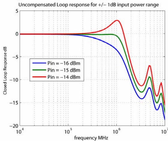
Figure 2: loop bandwidth vs. input level.
