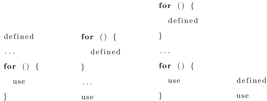
(a) use in a sub-loop of defined (b) define in a sub-loop of use (c) define and use in distinct loops (d) define and use in same loop
