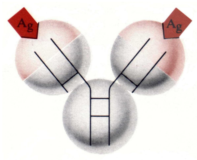
Figure 3. Stylized diagram of the three-dimensional structure of an IgG antibody molecule. Reprinted with permission from Pearson Education, Inc., Upper Saddle River, NJ 07458
