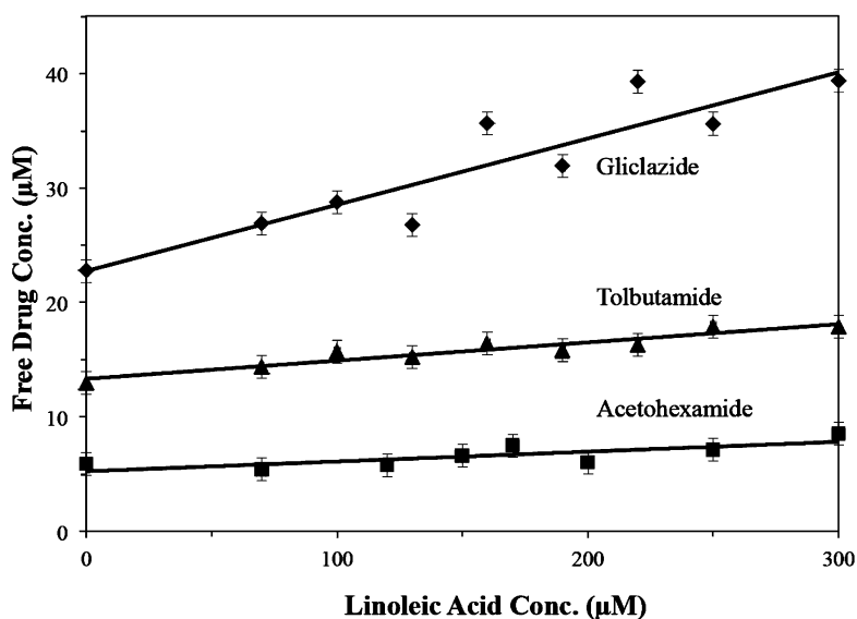
Figure 3. Effect of increasing the concentration of linoleic acid on the free drug concentration of acetohexamide (■), gliclazide (◆) and tolbutamide (▲) in the presence of fixed total concentrations of each drug and normal HSA. Each point represents the average of three measurements and the error bars represent a range of \pm 1 S.D.
