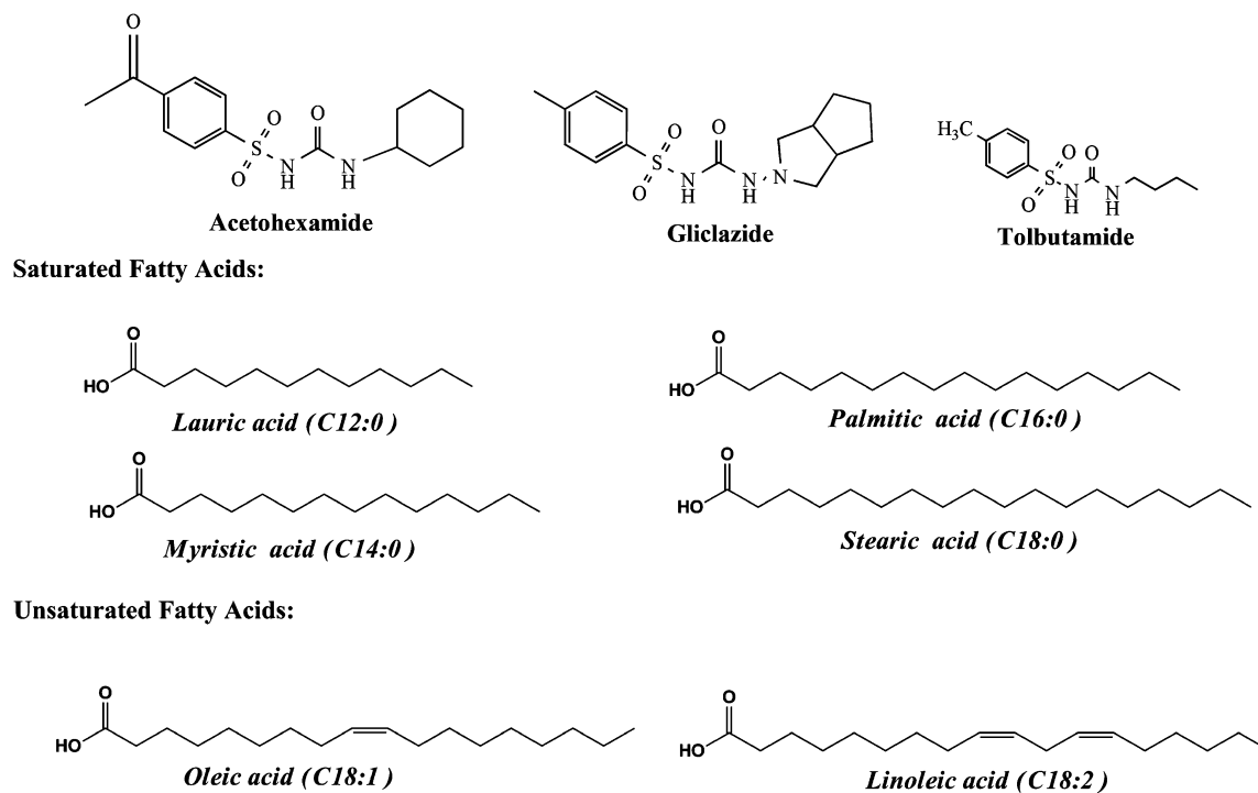
Figure 1. Structures of the sulfonyleurea drugs and fatty acids that were examined in this study.
