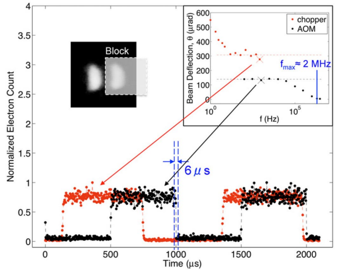
Figure 2. Electron counts as a function of time as the laser is switching on and off. Both chopper data (red dots) at 818 Hz and AOM data (black dots) at 1000 Hz are shown. Top-left inset: a time-averaged image shows the initial and deflected electron beam. A semi-transparent rectangle is added to depict a movable electron beam-stop. Top-right inset: the deflection magnitude \theta is plotted as a function of the chopping frequency f . The estimated maximum chopping frequency according our heuristic model, f_{\text{max}} \approx 2 \text{MHz} , is also drawn (blue line) for comparison. The red dots are data collected with a mechanical chopper and the black dots with an AOM.
