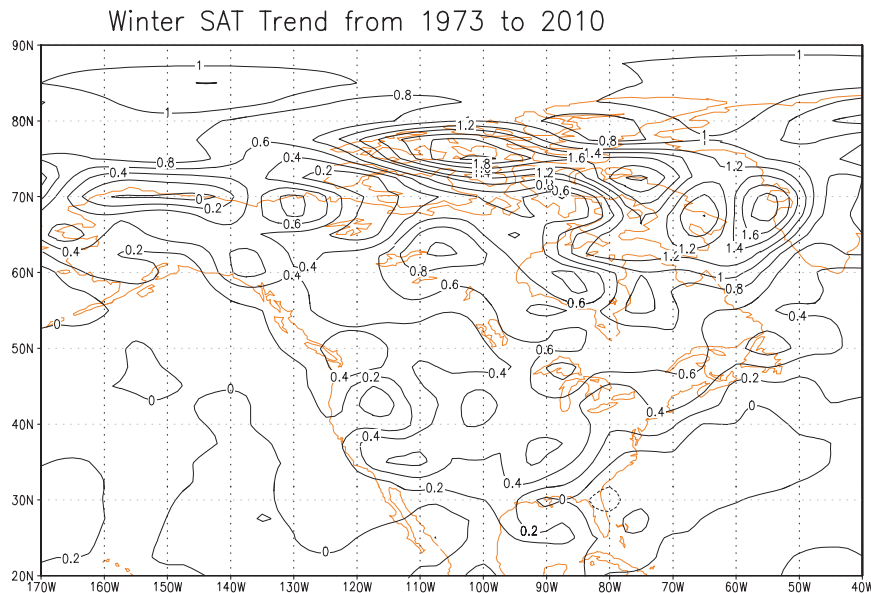
FIG. 7. Winter SAT trend ( ^{\circ}\text{C} \text{decade}^{-1} ) for the period 1973–2010, calculated using a least squares fit.
