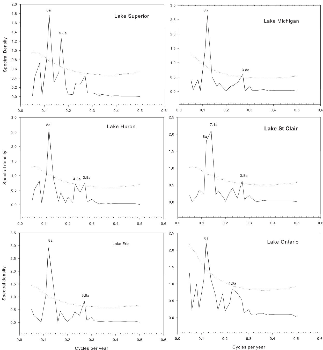
FIG. 6. Spectral analysis of LIA anomalies in all six lakes with the linear trends removed. The dotted curves are the 95% significance level. The peaks are marked with the corresponding periods in years.
