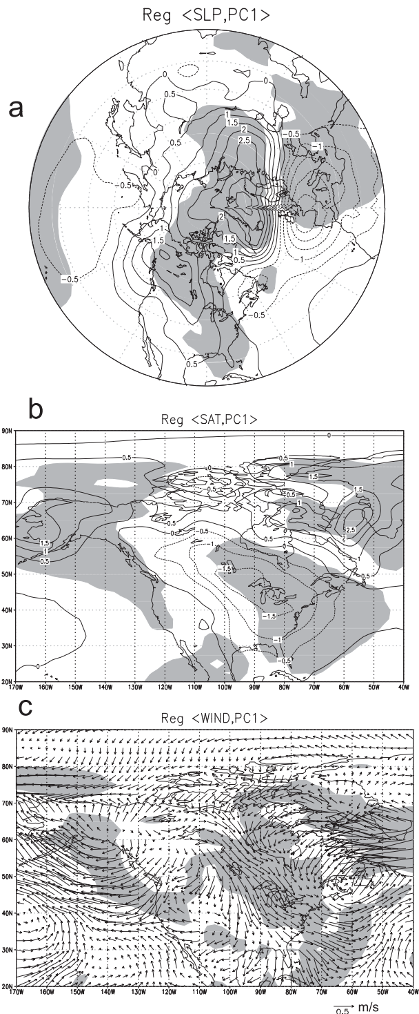
FIG. 9. The anomalous (a) SLP (hPa), (b) SAT ( ^{\circ}\text{C} ), and (c) surface wind ( \text{m s}^{-1} ) maps regressed to the time series of the first EOF mode of lake ice for the period 1973–2010. The shaded areas are over 95% significance level. Contour intervals for (a) SLP and (b) SAT are 0.5 hPa and 0.5^{\circ}\text{C} . The unit of anomalous winds in (c) is in 0.5 \text{ m s}^{-1} , as shown by the vector at the bottom.
