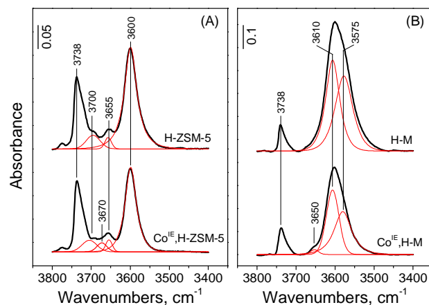
Fig. 9. DRIFT spectra of the \nu_{OH} region for (A) H-ZSM-5 and \text{Co}^{\text{IE}},\text{H-ZSM-5} sample and (B) H-M and \text{Co}^{\text{IE}},\text{H-M} sample (thick lines). The spectra were recorded in He flow at 573 K. Thin lines indicate the component bands obtained by a curve fitting computer program.
