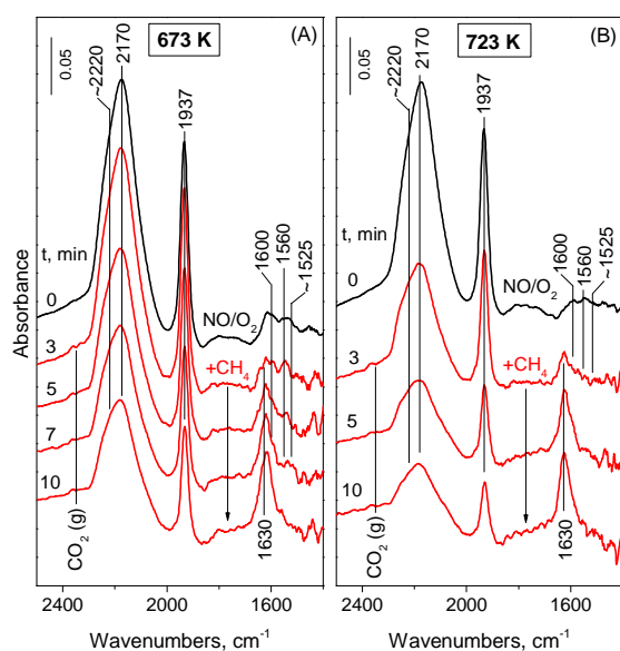
Fig. 10. Operando DRIFT spectroscopic examination of the transient response of the \text{Co}^{\text{SSR}},\text{Co}^{\text{IE}},\text{H-M}(1) catalyst on the change of the reactant composition. Catalyst was contacted with a flow of 4000 ppm NO/2% \text{O}_2/\text{He} at GHSV 30 000 \text{h}^{-1} at (A) 673 K and (B) 723 K. The first spectrum was recorded after the steady state was established (uppermost spectrum), then the flow was abruptly changed to a similar flow of 4000 ppm NO/4000 ppm \text{CH}_4 /2% \text{O}_2/\text{He} (indicated as + \text{CH}_4 ). Spectra were recorded after the given time on stream. The spectrum of the catalyst in He at the corresponding reaction temperature (673 K or 723 K) was subtracted from each spectrum and the difference spectra are shown.
