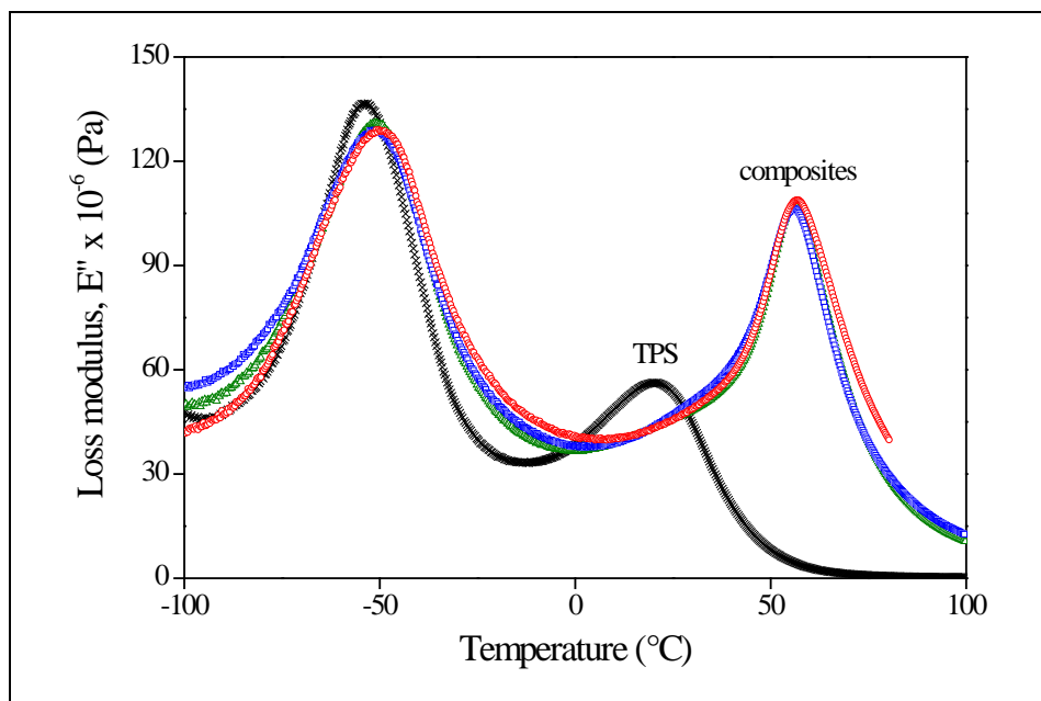
Fig. 4 Temperature dependence of the loss modulus of TPS and its wood composites at 30 vol% wood content; decreased mobility in the presence of wood; Symbols: ( \circ ) W126, ( \square ) W68, ( \triangle ) W35
