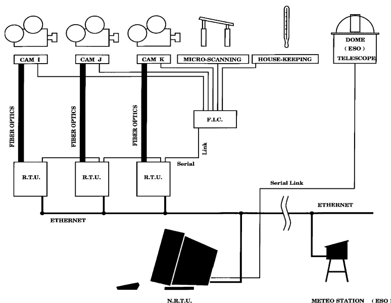
Figure 3: The DENIS computer network (from F. Lacombe).
