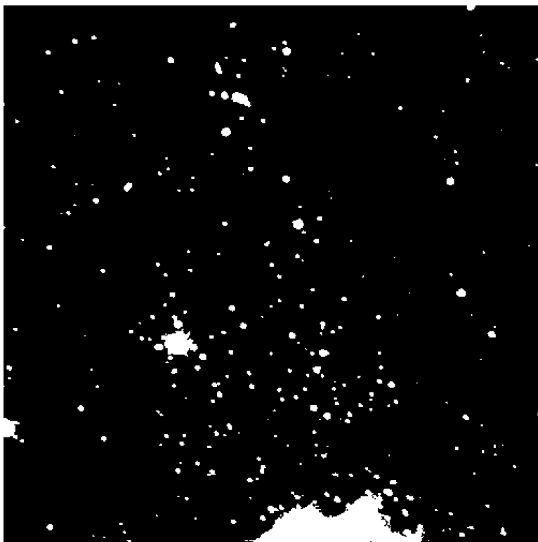
Figure 5: DENIS image of the molecular cloud OMC2 as seen in J and K_s (false colours, blue = J, red = K_s , processed by E. Copet).
