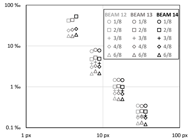
Figure 6. Principal strain resolution. Standard deviation, for the undeformed beam in terms of facet size, for different distance-to-size ratios.
