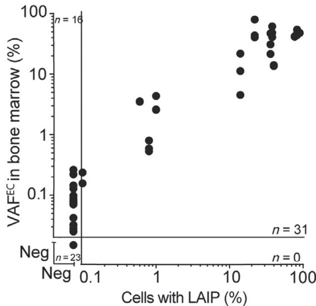
Figure 5.4: Comparison of determined MRD levels between targeted deep sequencing (y-axis) and MFC (x-axis). The lines shows the limit of detection at 0.020% for deep sequencing and 0.1% for MFC. Neg denotes a value below the limit of detection, LAIP denotes leukaemia-associated immunophenotype. Fifty-four determinations showed consistent MRD assignment (31 MRD + with both methods and 23 MRD - with both methods), while 16 determinations differed (all those were MRD + with deep sequencing and MRD - with MFC).
