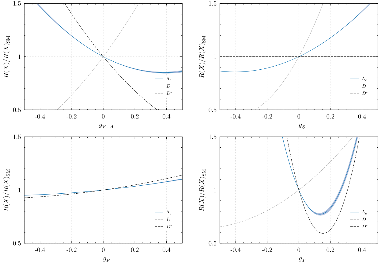
FIG. 7. R(\Lambda_c)/R(\Lambda_c)_{\text{SM}} and R(D^{(*)})/R(D^{(*)})_{\text{SM}} predictions for real NP couplings, in the operator basis of Eq. (3).
