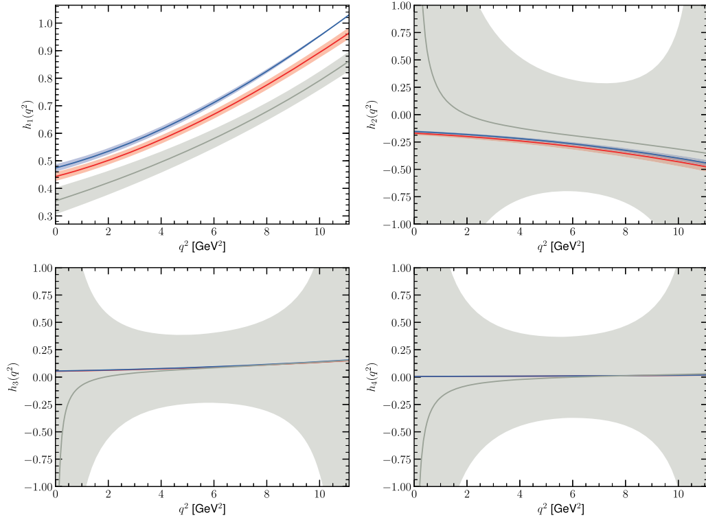
FIG. 4. Predictions for the tensor form factors based on Eq. (13) and our fit to the LHCb data and the LQCD calculation of the (axial) vector form factors, overlaid on the LQCD calculation of the tensor form factors [51] (gray bands; scaled to \mu = \sqrt{m_b m_c} ). The red bands show our nominal fit including \Lambda_{\text{QCD}}^2/m_c^2 terms; the blue bands show fit results with \Lambda_{\text{QCD}}^2/m_c^2 terms set to zero.
