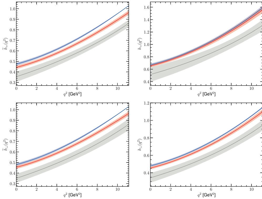
FIG. 5. Predictions for the tensor form factors in the basis used in the LQCD calculation [51] (gray bands, scaled to \mu = \sqrt{m_b m_c} ), compared with our predictions based on Eq. (13) and the fit to the LHCb data and the LQCD (axial)vector form factors. The red bands show our nominal fit including \Lambda_{\text{QCD}}^2/m_c^2 terms; the blue bands show fit results with \Lambda_{\text{QCD}}^2/m_c^2 terms set to zero.
