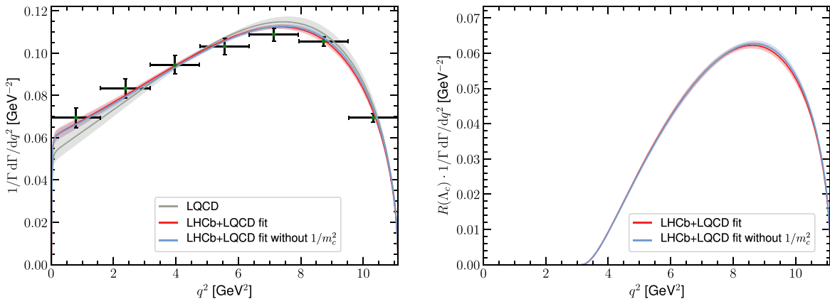
FIG. 1. Left: The data points show the LHCb measurement of the normalized d\Gamma(\Lambda_b \rightarrow \Lambda_c \mu\bar{\nu})/dq^2 spectrum [2]. The red band shows our fit of the HQET predictions to these data [2] and to the LQCD form factors [3]. The blue curve shows the fit results, setting the order \Lambda_{\text{QCD}}^2/m_c^2 terms to zero. The gray band shows the LQCD prediction. Right: Our prediction for d\Gamma(\Lambda_b \rightarrow \Lambda_c \tau\bar{\nu})/dq^2 normalized to R(\Lambda_c) from the same fit, with and without including the \Lambda_{\text{QCD}}^2/m_c^2 terms.
