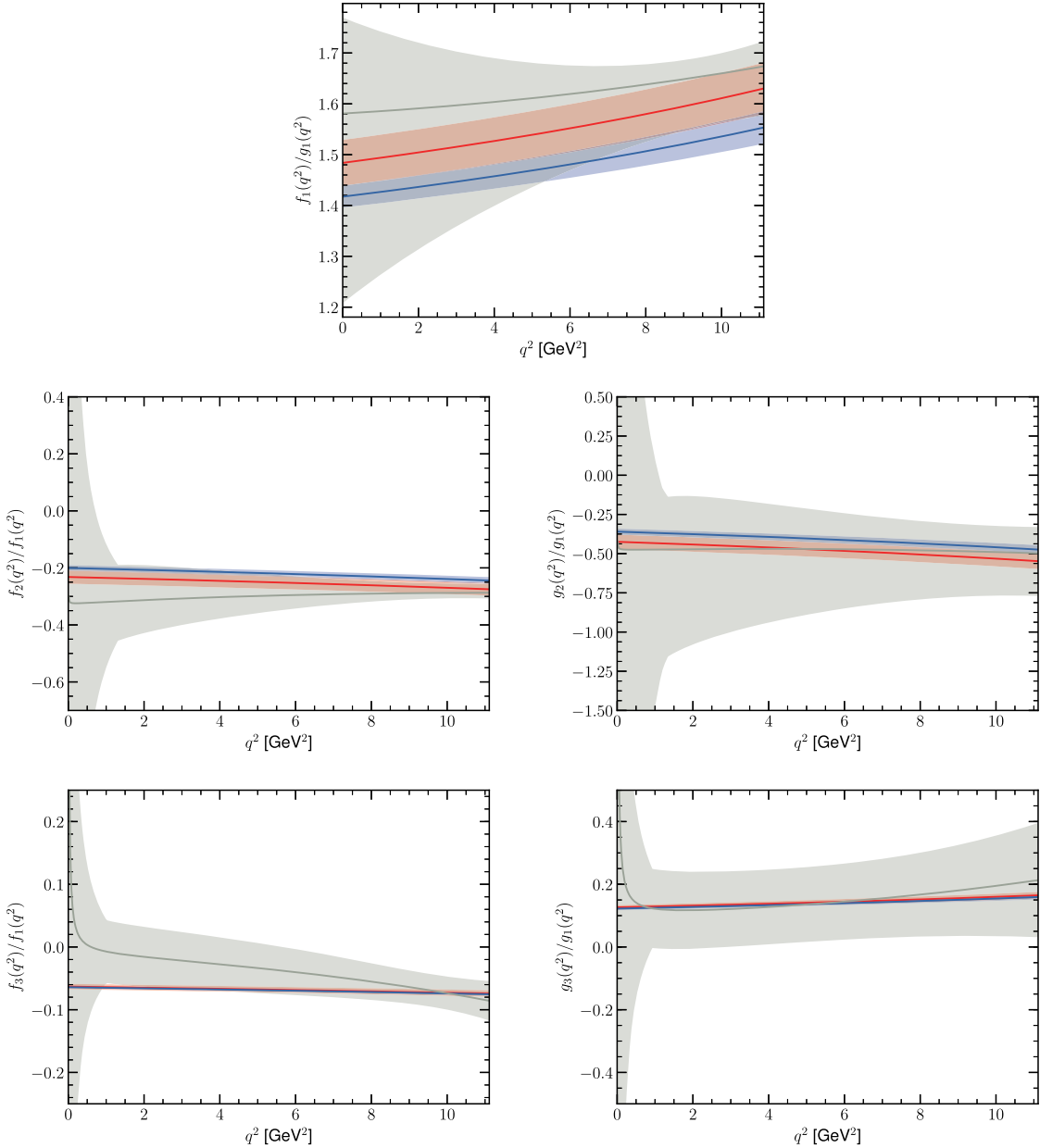
FIG. 3. Fits of the HQET predictions in Eq. (12) to the LQCD results [3] (gray bands), for five ratios of the six form factors. The top row shows f_1/g_1 , which is \mathcal{O}(1) in HQET, whereas f_{2,3}/f_1 (left column) and g_{2,3}/g_1 (right column) are expected to be \mathcal{O}(\alpha_s, \Lambda_{\text{QCD}}/m_Q) . The red bands show our nominal fit including \Lambda_{\text{QCD}}^2/m_c^2 terms; the blue bands show fit results with \Lambda_{\text{QCD}}^2/m_c^2 terms set to zero.
