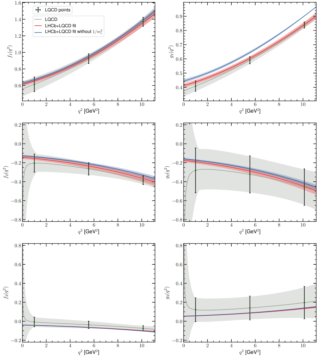
FIG. 2. Fits of the HQET predictions in Eq. (12) to the LQCD results [3] for the six form factors (red bands) for f_{1,2,3} (left column) and g_{1,2,3} (right column). The blue bands show the same fits, setting the order \Lambda_{\text{QCD}}^2/m_c^2 terms to zero. Also shown are the LQCD predictions (gray bands and data points); see text for details.
