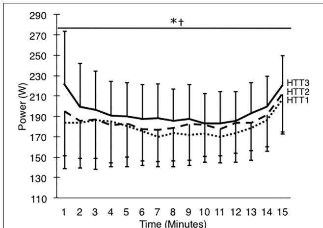
FIGURE 4 | Power output (W) during 15-min time trials in hot conditions (35°C, 30% RH) performed pre-acclimation (HTT1; dotted line), following 4-days heat acclimation (HTT2; dashed line), and following 9-days heat acclimation (HTT3; solid line). Each data point is an average of the preceding minute, and presented as mean ± SD. Significant effect of condition: *HTT3 > HTT1 ( p < 0.05 ), †HTT3 > HTT2 ( p < 0.05 ).
