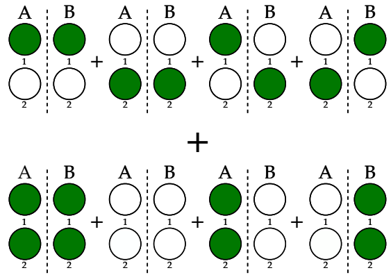
FIG. 1. Depiction of the eight even number parity fermion states of four single-particle modes, partitioned such that the two modes on the left of the dashed line belong to Alice, whereas the two modes on the right to Bob. The upper row are the states with odd local number parity (one fermion for Alice and one fermion for Bob) whereas the bottom row those with even local number parity (Alice and Bob may have 0 or two fermions). The states of the bottom row can be formally obtained from those on the top by performing particle-hole transformations c_{A_2}^\dagger \leftrightarrow c_{A_2} and c_{B_2}^\dagger \leftrightarrow c_{B_2} .
