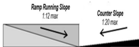
Figure 2: Curb Ramps (CR) Slope's Details
