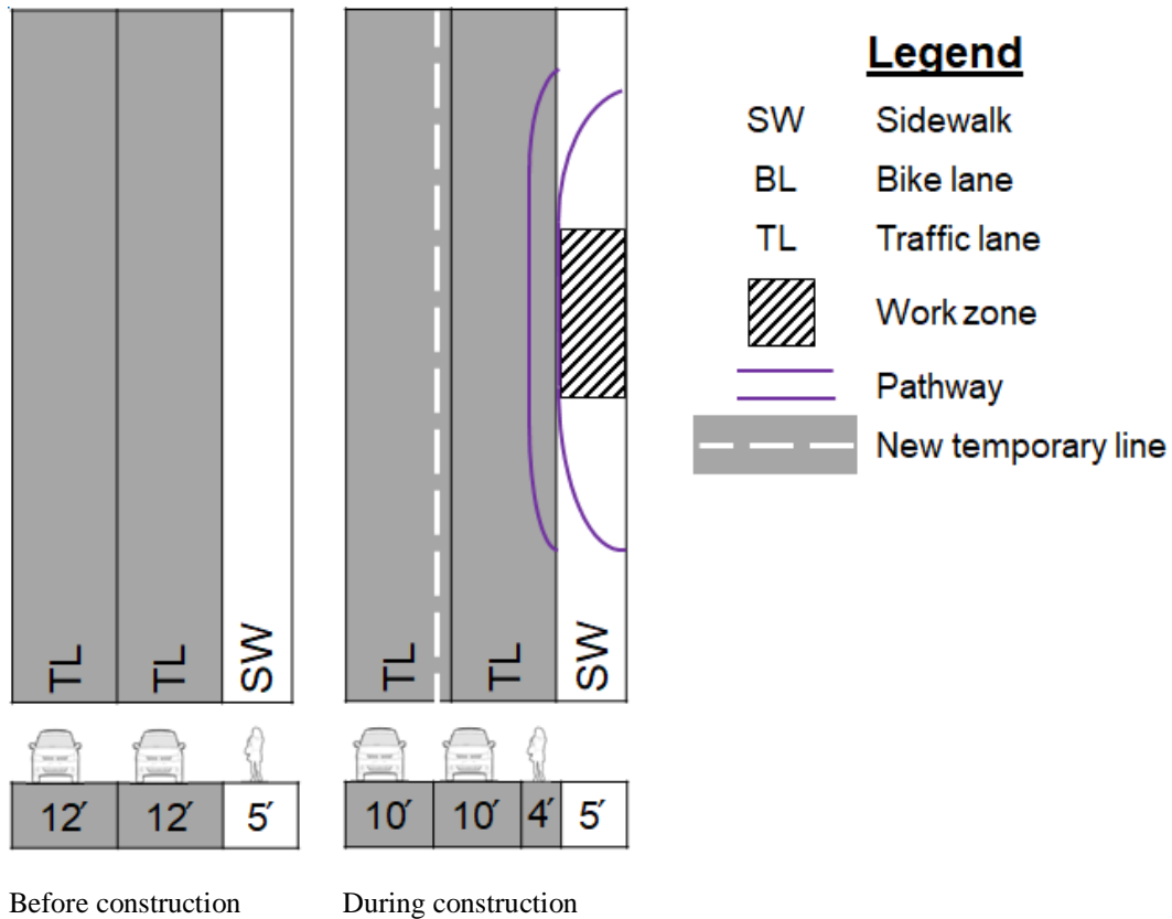
Figure 4-8. Pathway on a traffic lane
