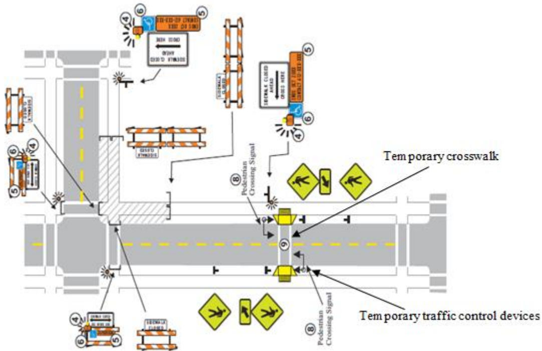
Figure 4-15. Temporary crosswalk (MN MUTCD 2015)
