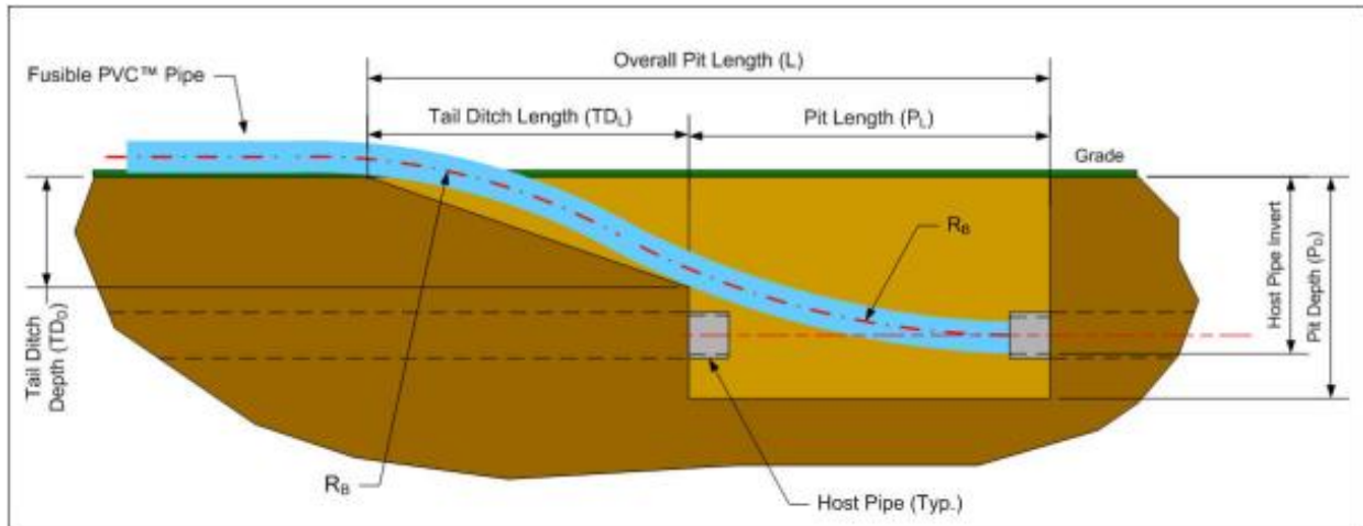
Figure 2-23. Typical sliplining, boring, and/or pipe bursting insertion/receiving pit (Underground Solutions 2016)
