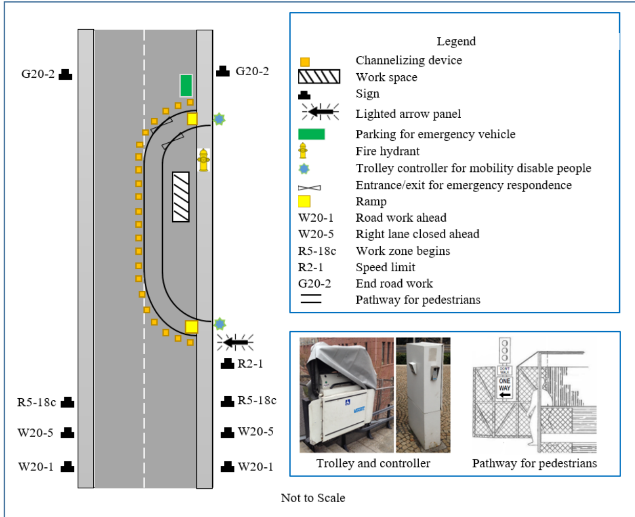
Figure 4-12. Typical layout and signage of a construction site
