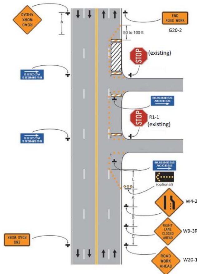
Figure 4-14. Alternatives to provide access to businesses during construction (Porter et al. 2016)
