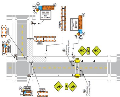
Figure 1-6. Fences to separate non-motorized traffic from work zone and live traffic
