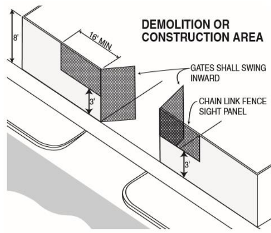
b) A typical construction site with tall fences (Slcdocs 2017)
