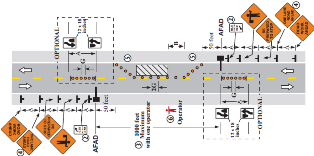
c) Typical layout of using AFAD in two-lane two-way road
