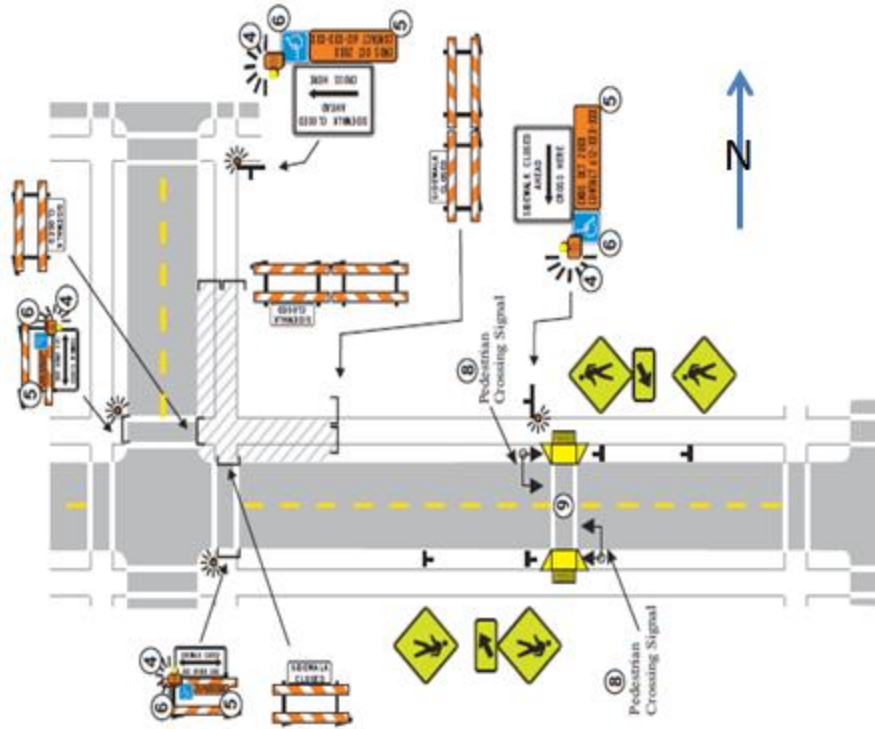
Figure 2-6. Temporary crosswalk (MN MUTCD 2015)
