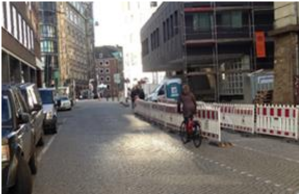
a) A temporary bicycle lane and a walkway
