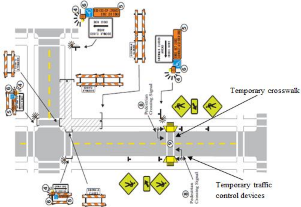
a) Temporary crosswalk (MN MUTCD 2015)
