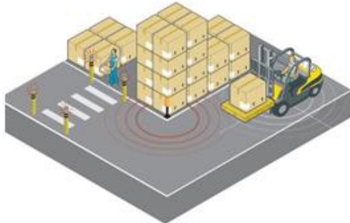
Figure 2-34. Crossing alert-pedestrian warning system (ZoneSafe 2017)
