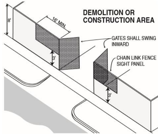
b) A typical construction zone with tall fences (Slcdocs 2017)
