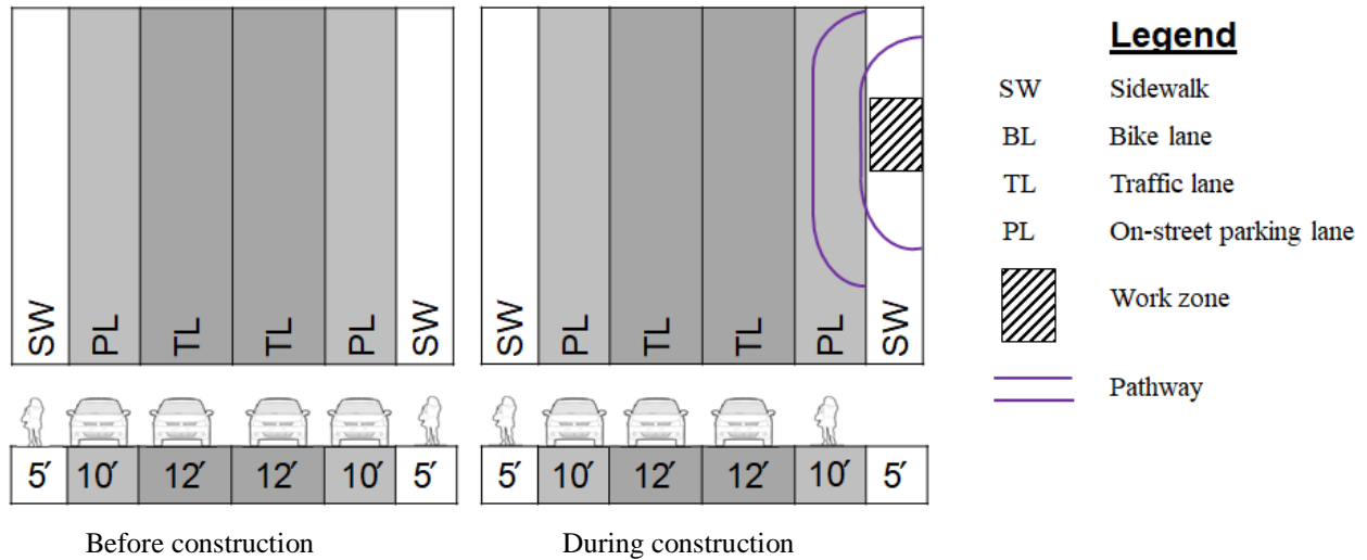
Figure 4-4. Non-motorized pathway located within an on-street parking lane
