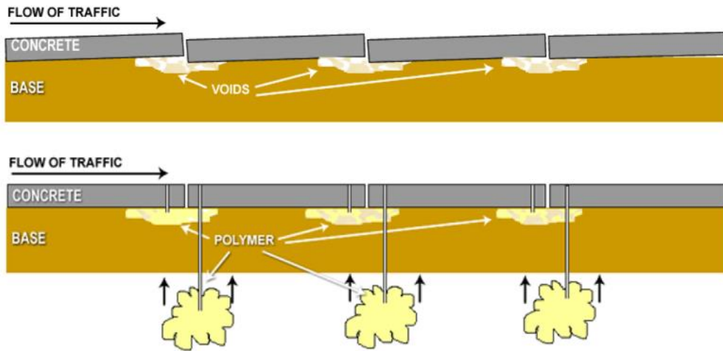
a) Slab jacking, slab stabilization, and soil densification process (Barrette 2014)
