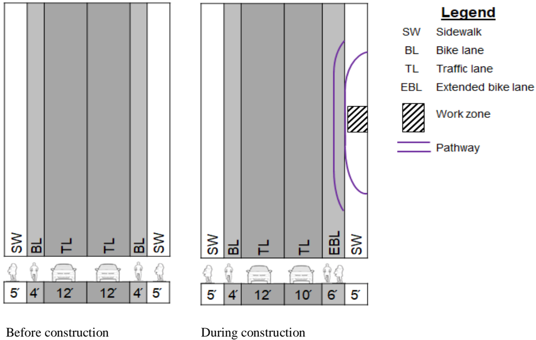
Figure 4-7. Pathway on an extended bike lane
