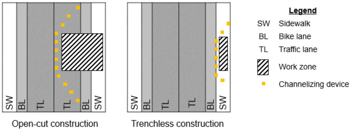
b) Space requirement for open-cut and trenchless construction.
