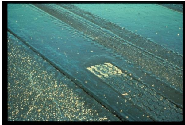
Figure 2-28. Traditional bond coat (Sherocman 2015)
