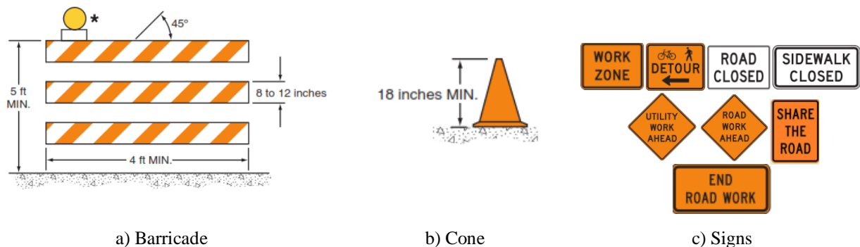
Figure 2-2. TTC devices (MUTCD 2009)
