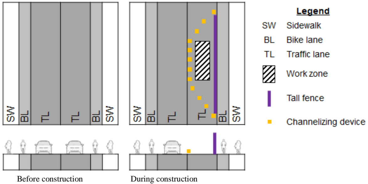
a) Work zone is located within a traffic lane
