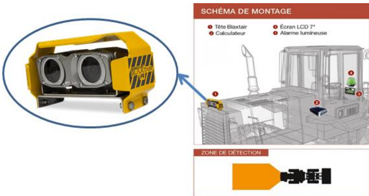
Figure 2-36. Blaxtair anti-collision camera (Blaxtair 2017)
