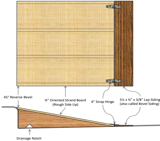
c) A ramp made of wood (Sinclair 2017)
