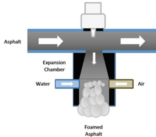
a) Warm mix asphalt (WMA) foaming process (Newcomn et al. 2015)
