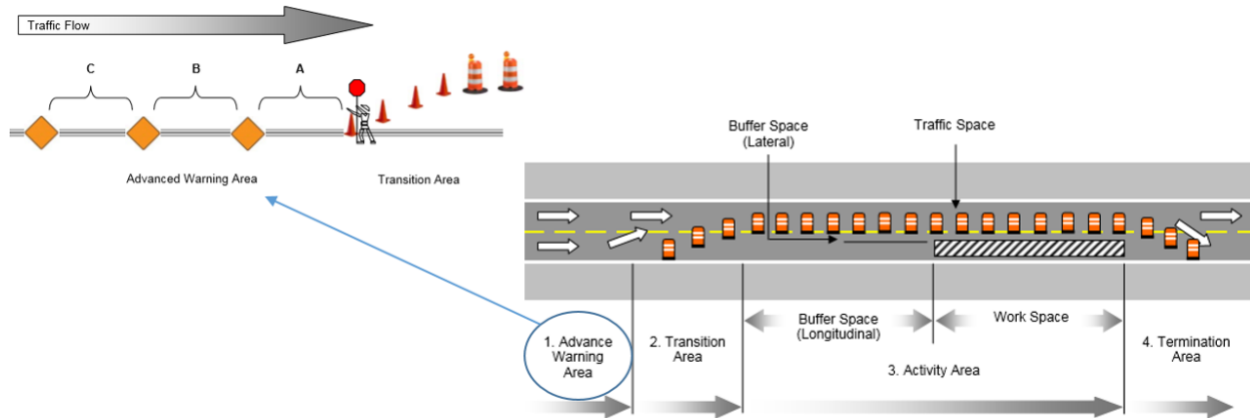
Figure 2-1. TTC zone components (MUTCD 2009, OSHA 2008)
