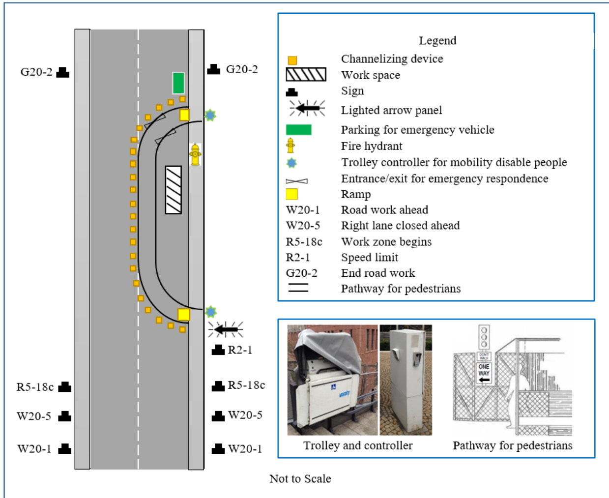
Figure C- 5. A typical site layout and access management for emergency responders
