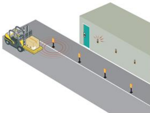
Figure 2-35. Walkway alert-approaching vehicle warning system (Zonesafe 2017)
