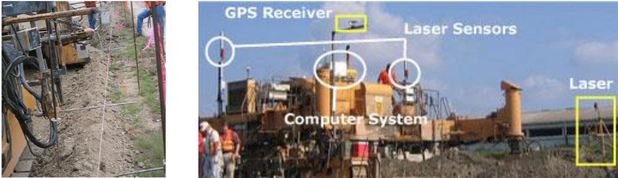
a) Stringlines and on-paver sensors
