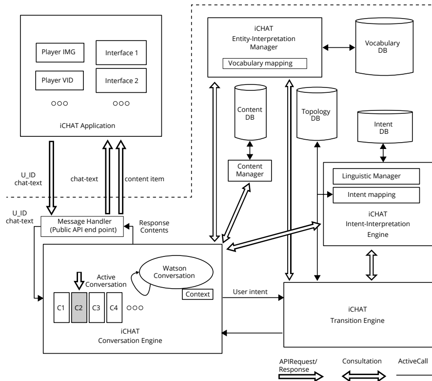
Figure 36. iCHAT's conversation manager architecture
