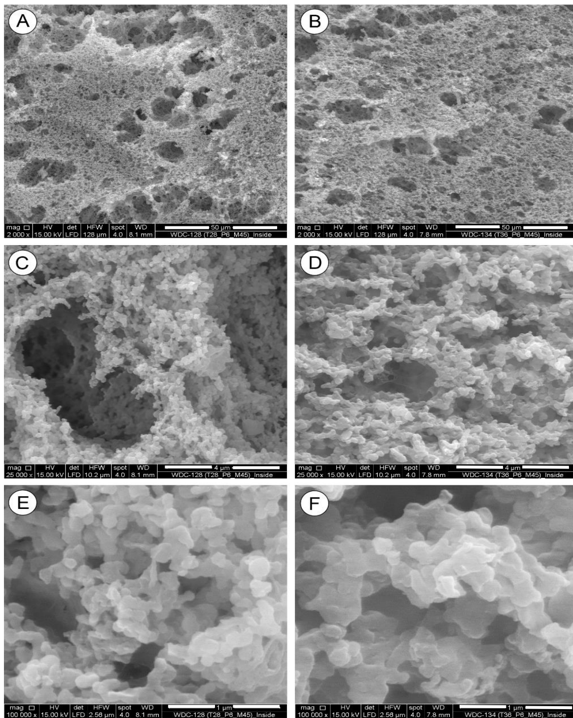
Figure 5.8 Representative scanning electron micrographs of cooked curd particles made from 6% protein-standardized milk that were renneted at two different set temperatures (A, C, E: 28°C; B, D, F: 36°C). Micrographs were taken at a distance of ~500 μm from the outside of the particle. Scale bars A, B = 50 μm, C, D = 4 μm and E, F = 1 μm.
