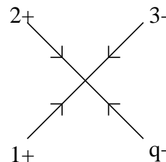
Figure 5: The (+, +, -, -) graviton vertex.
