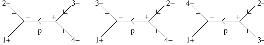
Figure 3: The MHV diagrams contributing to the \mathcal{M}(1+, 2-, 3-, 4-) graviton amplitude.
