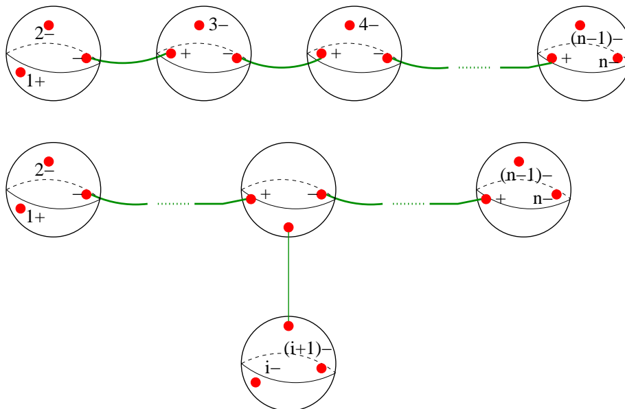
Figure 1: Two disconnected configurations contributing to \mathcal{M}_n(1+, 2-, \dots, n-) .
