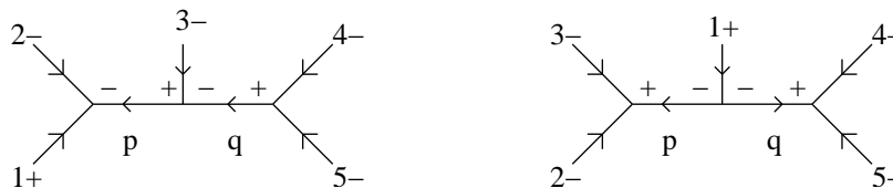
Figure 4: Two of the fifteen MHV diagrams contributing to the \mathcal{M}(1+, 2-, 3-, 4-, 5-) graviton amplitude.
