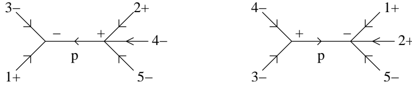
Figure 6: Two of the nine MHV diagrams contributing to the \mathcal{M}(1+, 2+, 3-, 4-, 5-) graviton amplitude.
