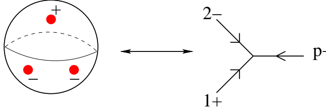
Figure 2: The (+, -, -) graviton vertex.
