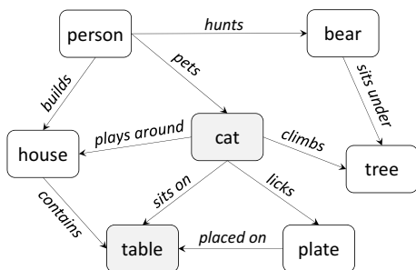
Figure 2: A toy knowledge graph modeling seven concepts as nodes (e.g., cat and table ), as well as their relationships as edges (e.g., “ cat sits on table ”).
